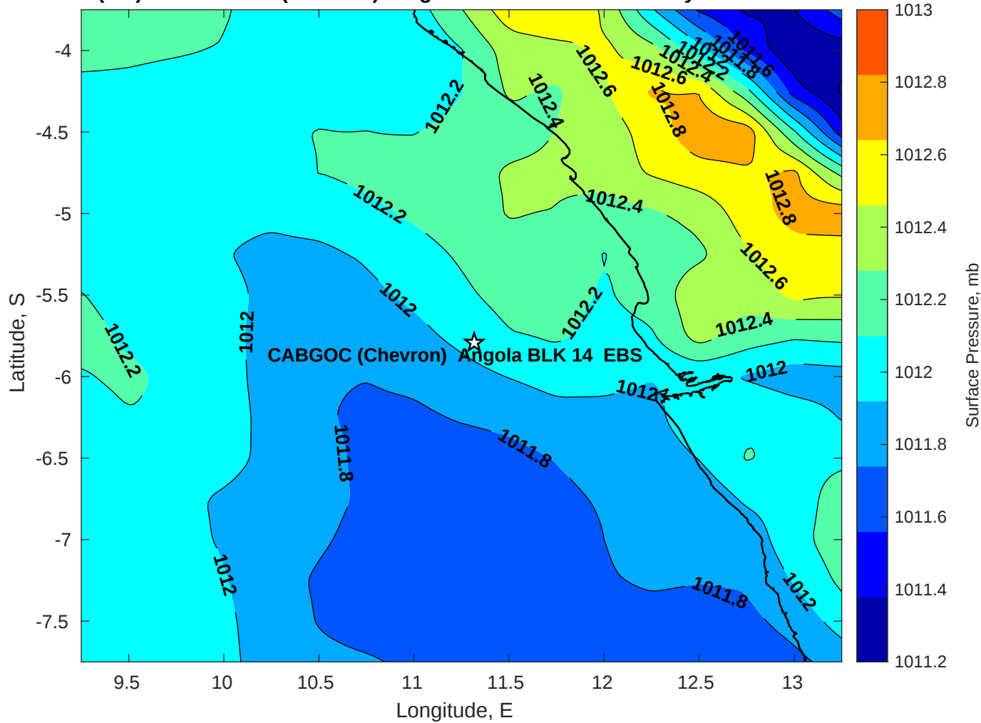
Surface Pressure (mb) for CABGOC (Chevron) Angola BLK 14 EBS at 24-May-2025 00:00:00
