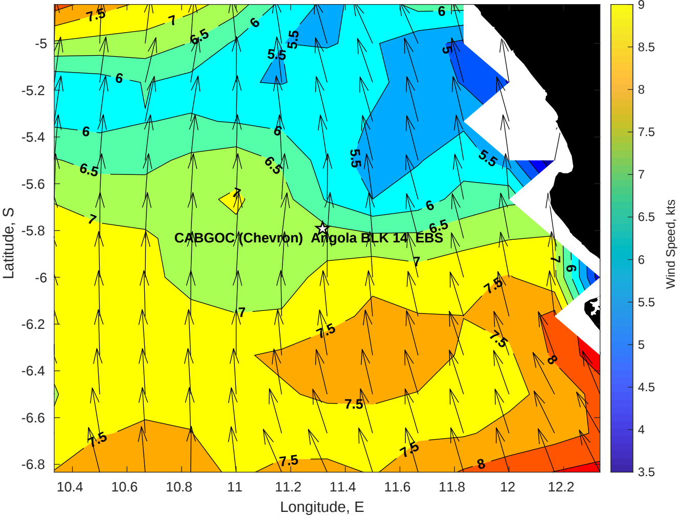
Winds (kts) for CABGOC (Chevron) Angola BLK 14 EBS at 24-May-2025 09:00:00
