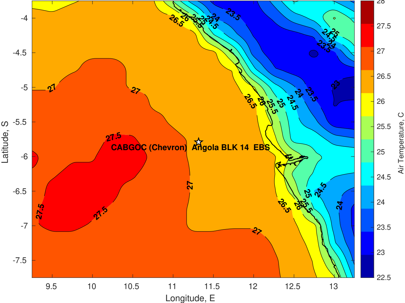
Air Temperature (C) for CABGOC (Chevron) Angola BLK 14 EBS at 24-May-2025
