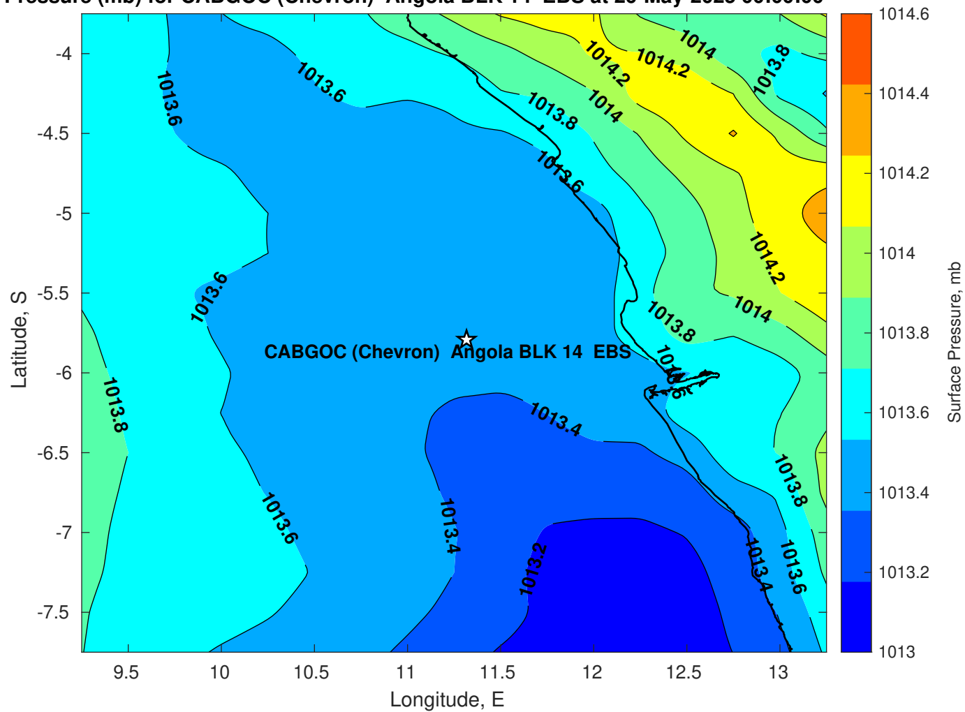
Surface Pressure (mb) for CABGOC (Chevron) Angola BLK 14 EBS at 26-May-2025 00:00:00
