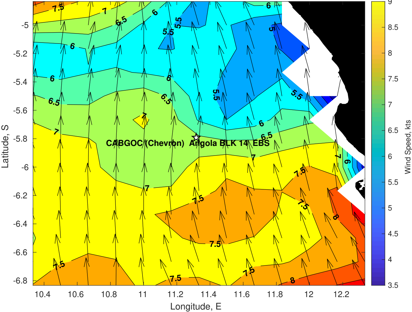
Winds (kts) for CABGOC (Chevron) Angola BLK 14 EBS at 24-May-2025 09:00:00
