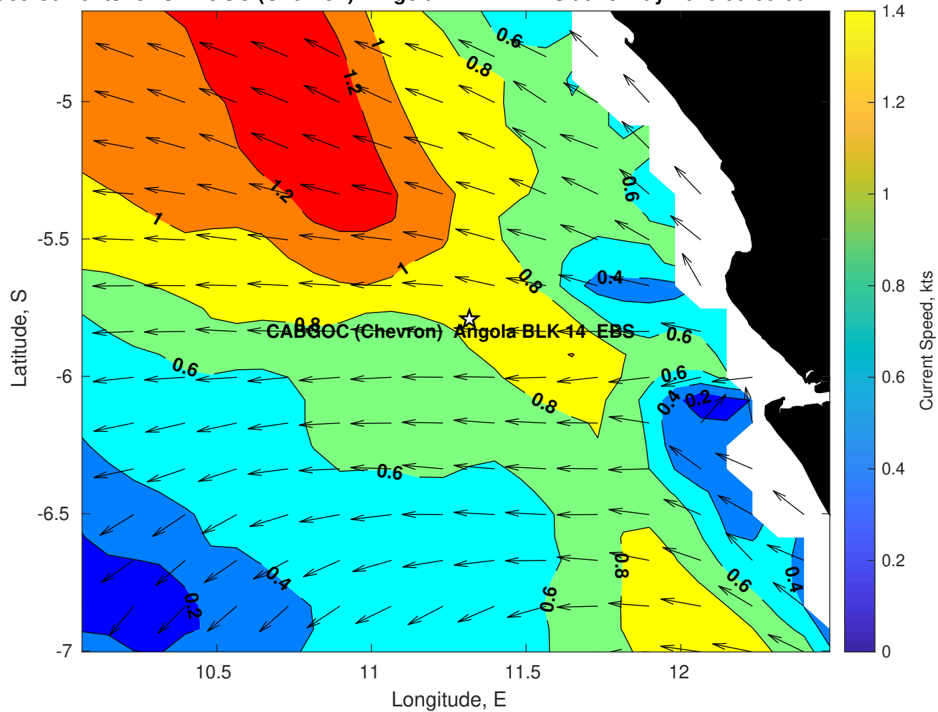
Surface Currents for CABGOC (Chevron) Angola BLK 14 EBS at 23-May-2025 00:00:00
