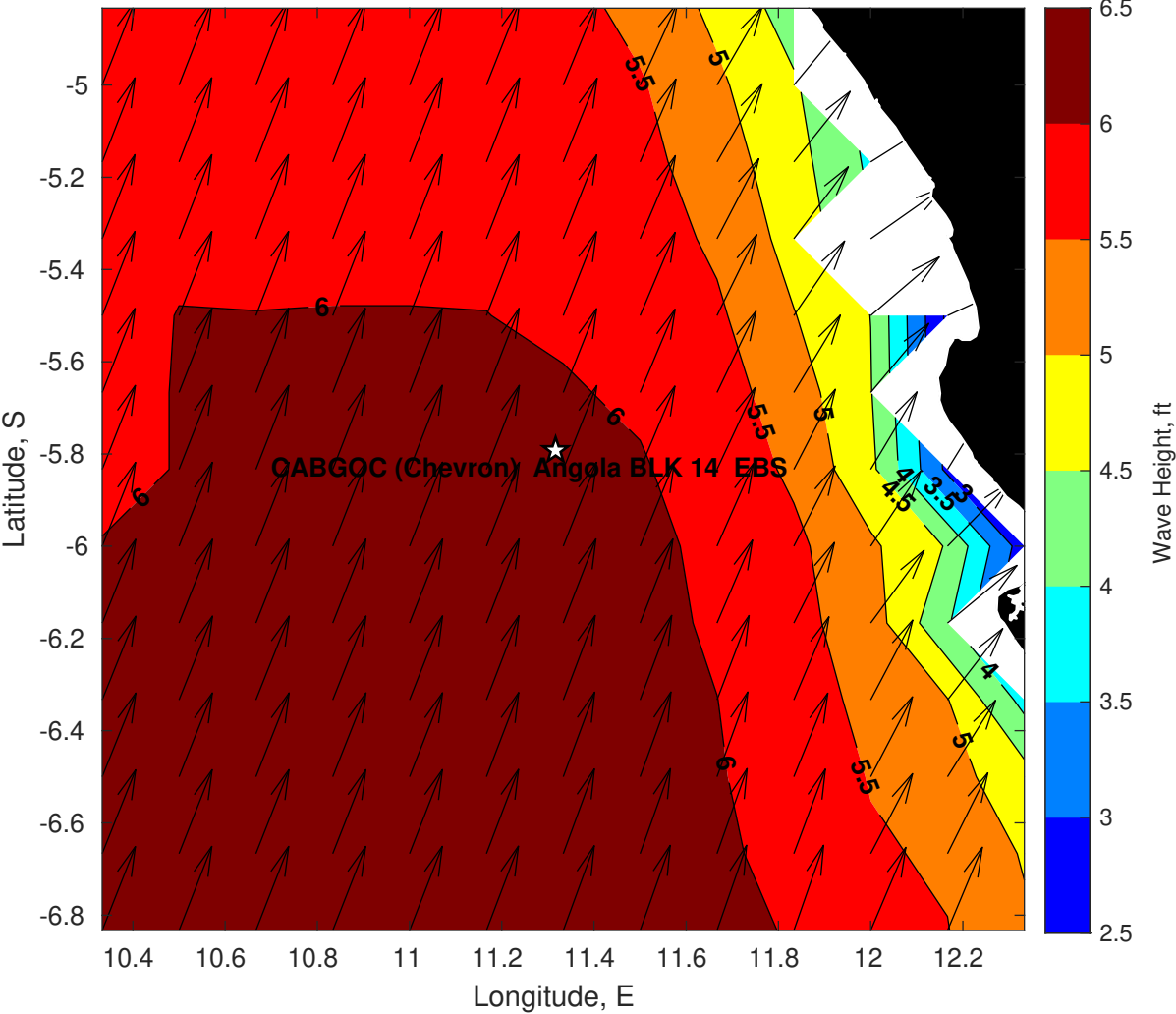
Wave Height (ft) for CABGOC (Chevron) Angola BLK 14 EBS at 24-May-2025 09:00:00
