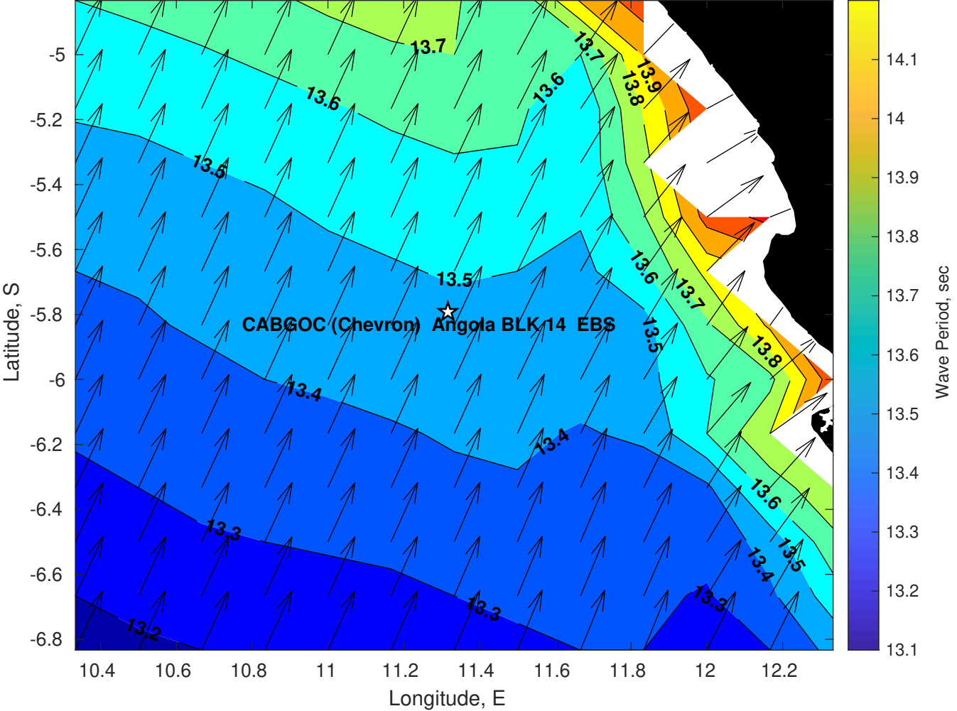
Wave Period (sec) for CABGOC (Chevron) Angola BLK 14 EBS at 24-May-2025 09:00:00
