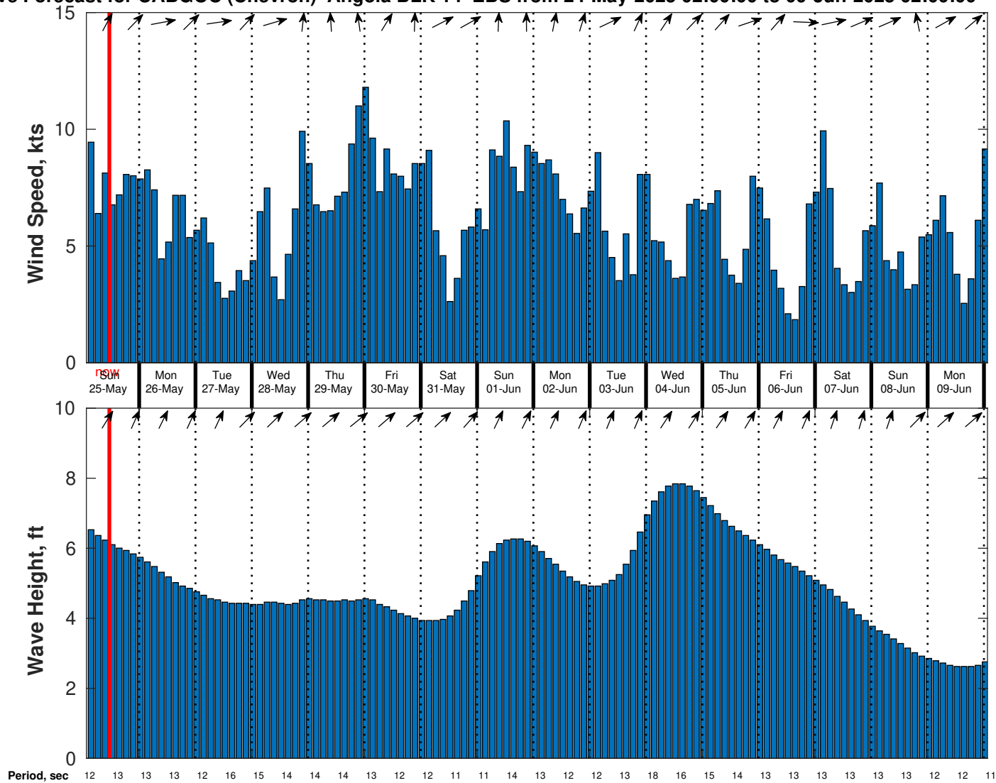
Wind & Wave Forecast for CABGOC (Chevron) Angola BLK 14 EBS from 24-May-2025 02:00:00 to 09-Jun-2025 02:00:00
