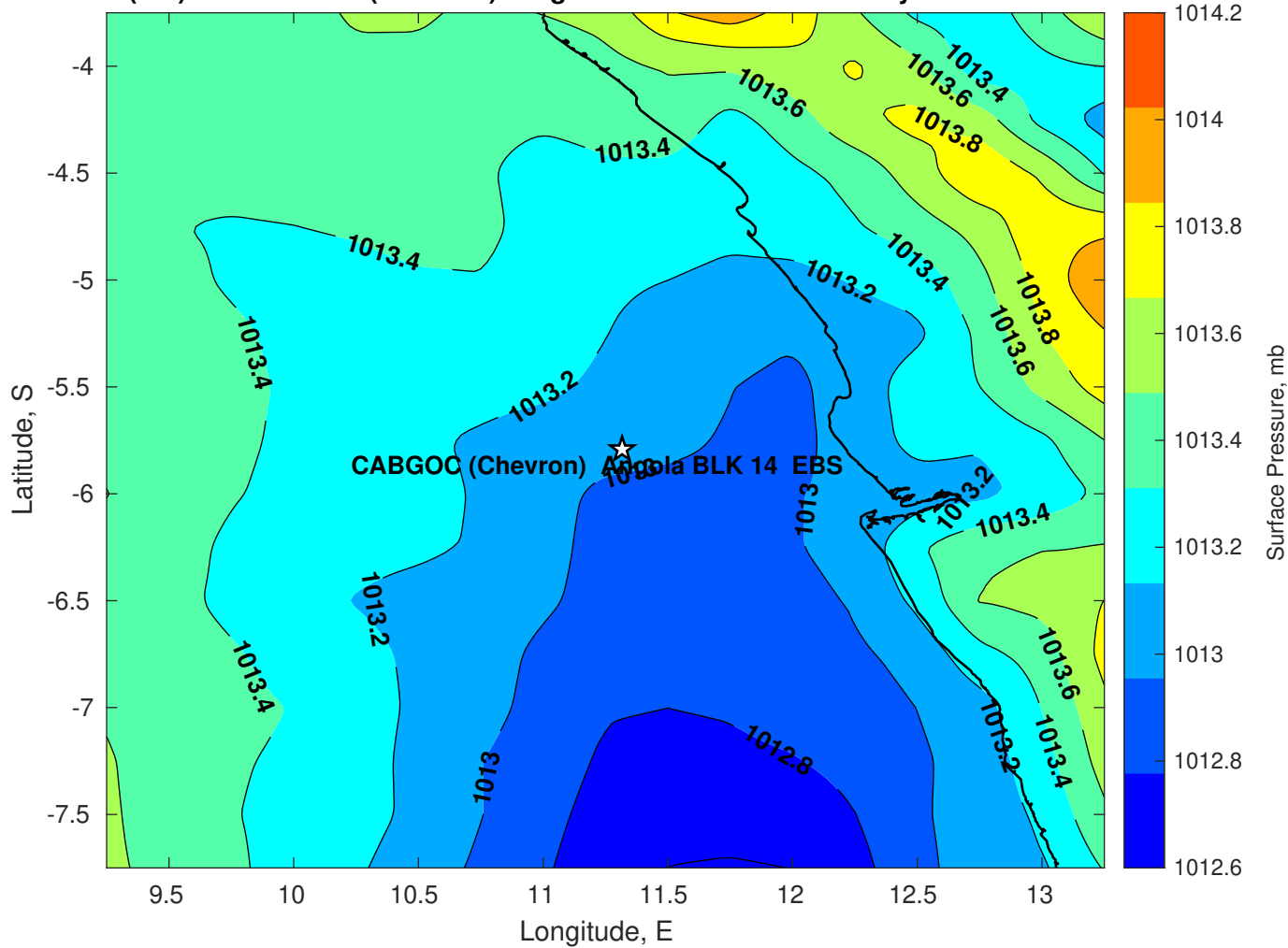
Surface Pressure (mb) for CABGOC (Chevron) Angola BLK 14 EBS at 25-May-2025 00:00:00
