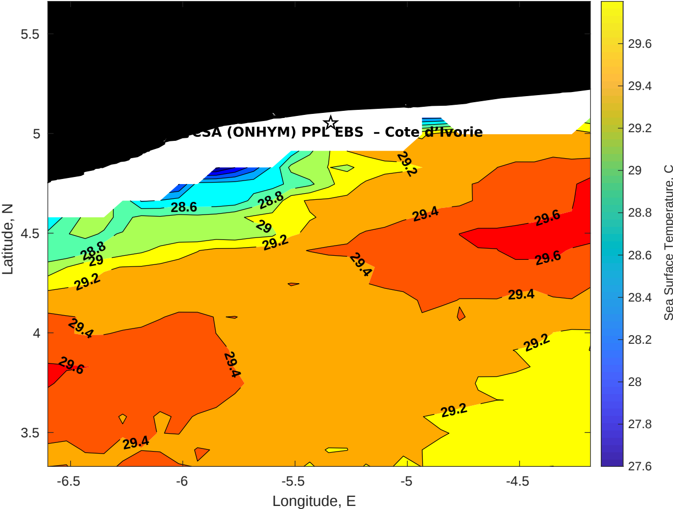
SST for CSA (ONHYM) PPL EBS - Cote d'Ivoire at 23-May-2025 00:00:00
