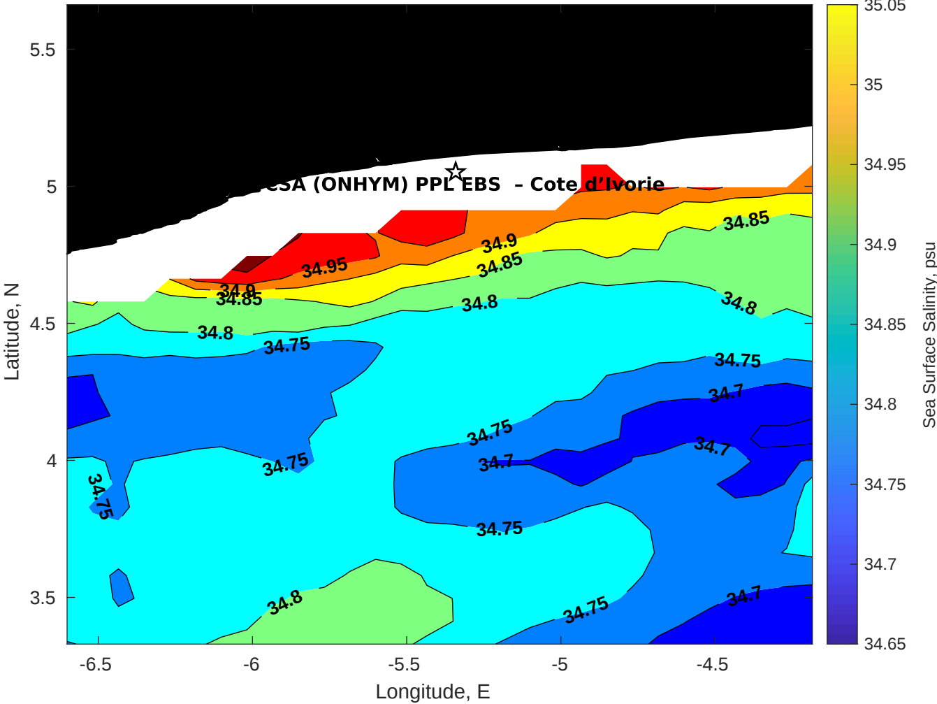
Surface Salinity for CSA (ONHYM) PPL EBS - Cote d'Ivoire at 23-May-2025 00:00:00
