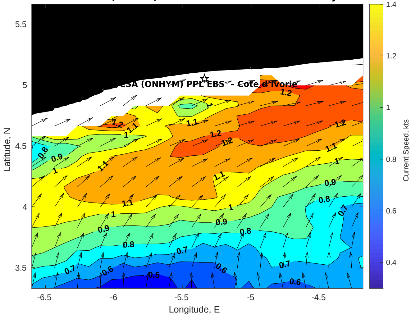
Surface Currents for CSA (ONHYM) PPL EBS - Cote d'Ivoire at 23-May-2025 00:00:00
