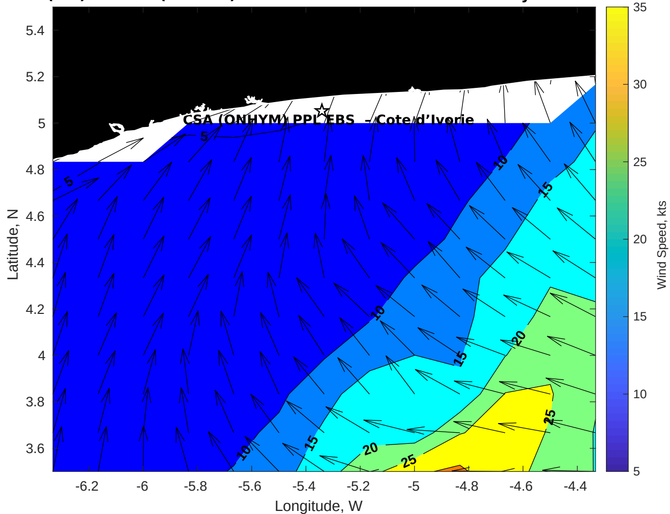
Winds (kts) for CSA (ONHYM) PPL EBS - Cote d'Ivoire at 24-May-2025 09:00:00
