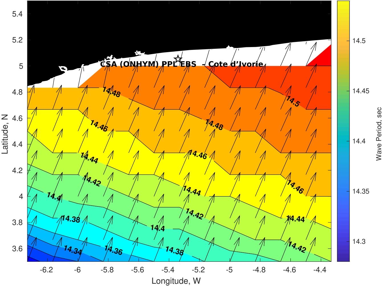
Wave Period (sec) for CSA (ONHYM) PPL EBS - Cote d'Ivoire at 24-May-2025 09:00:00
