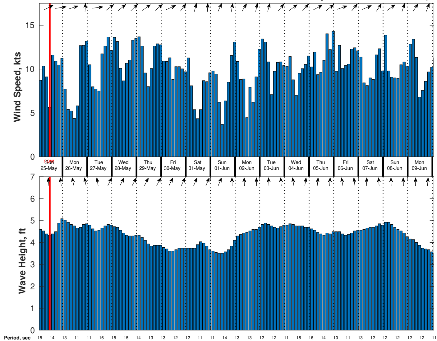
Wind & Wave Forecast for CSA (ONHYM) PPL EBS - Cote d'Ivoire from 24-May-2025 01:00:00 to 09-Jun-2025 01:00:00
