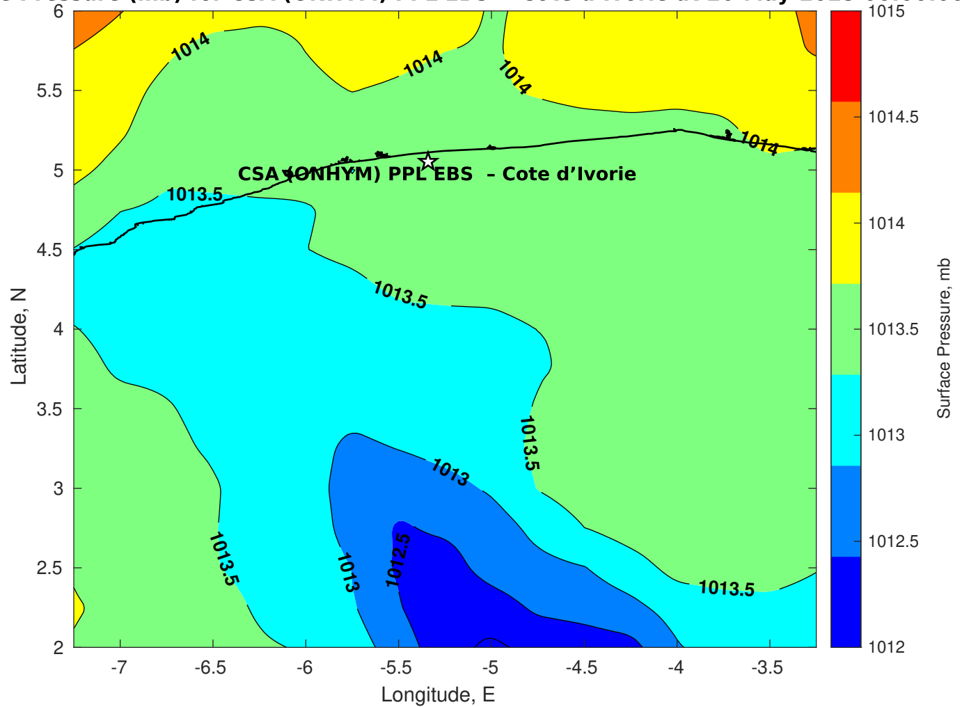
Surface Pressure (mb) for CSA (ONHYM) PPL EBS - Cote d'Ivoire at 26-May-2025 00:00:00
