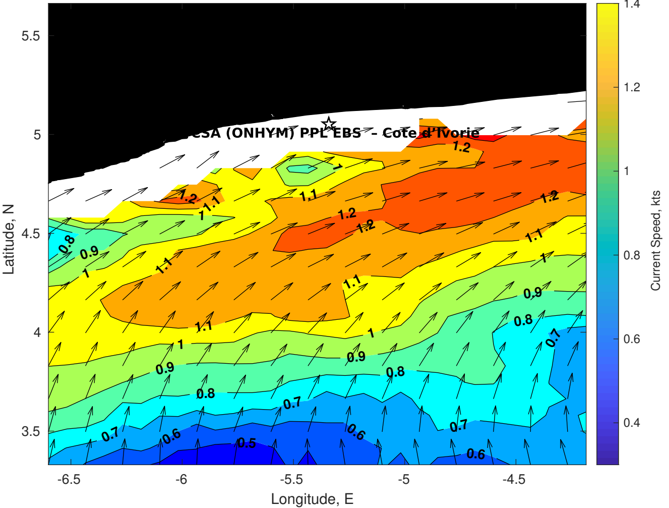
Surface Currents for CSA (ONHYM) PPL EBS - Cote d'Ivoire at 23-May-2025 00:00:00
