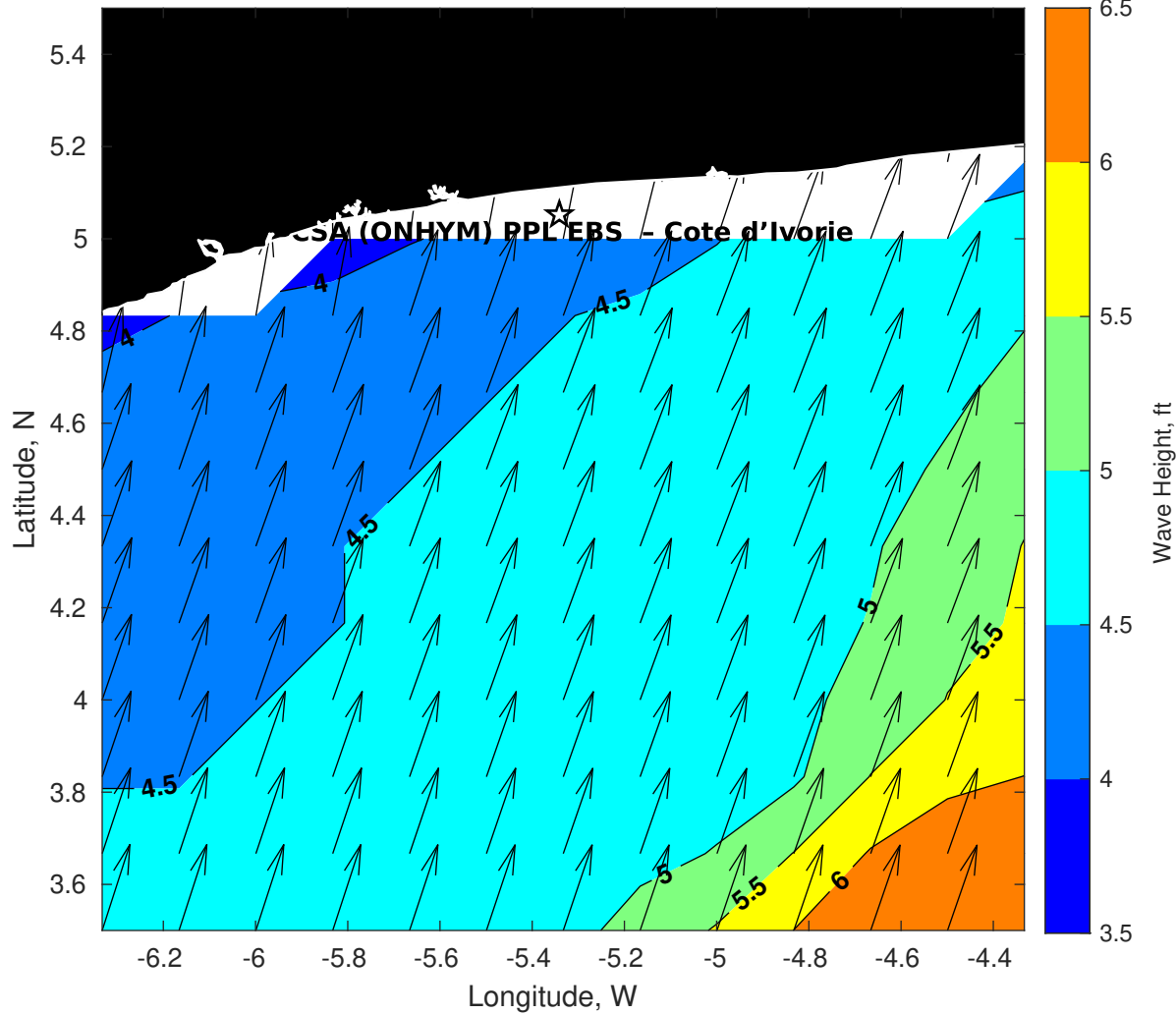
Wave Height (ft) for CSA (ONHYM) PPL EBS - Cote d'Ivoire at 24-May-2025 09:00:00
