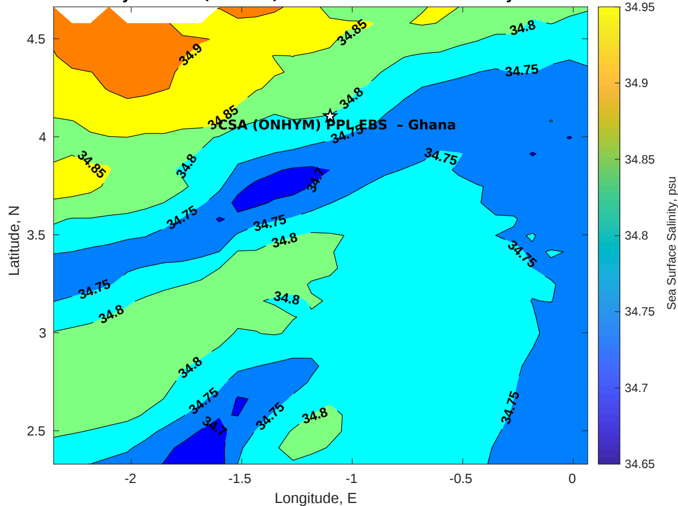
Surface Salinity for CSA (ONHYM) PPL EBS - Ghana at 23-May-2025 00:00:00
