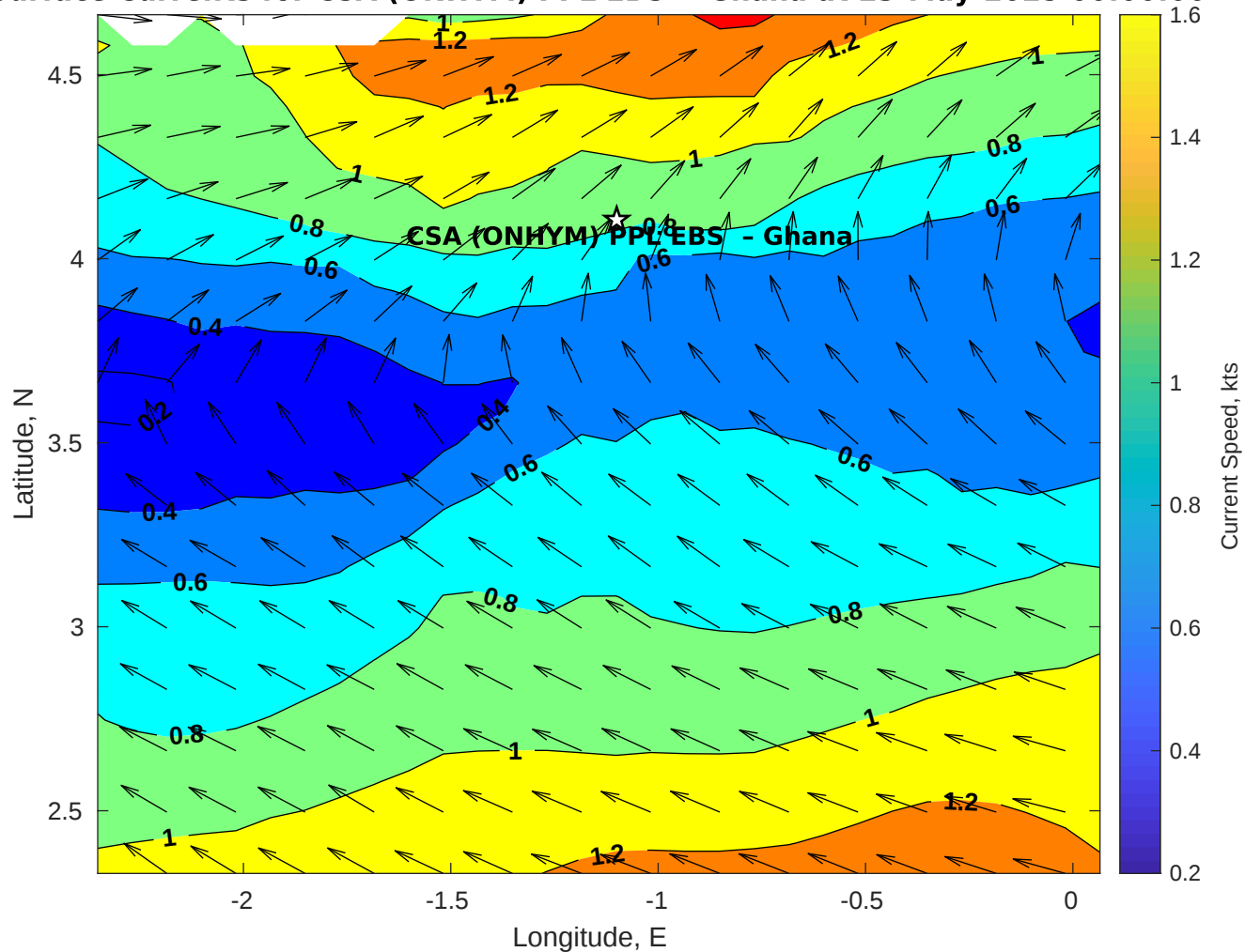
Surface Currents for CSA (ONHYM) PPL EBS - Ghana at 23-May-2025 00:00:00
