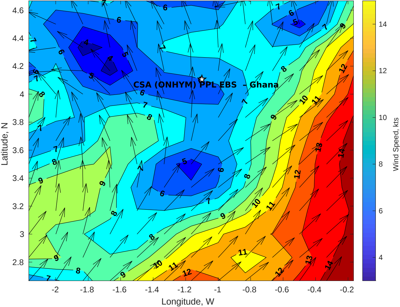
Winds (kts) for CSA (ONHYM) PPL EBS - Ghana at 24-May-2025 09:00:00
