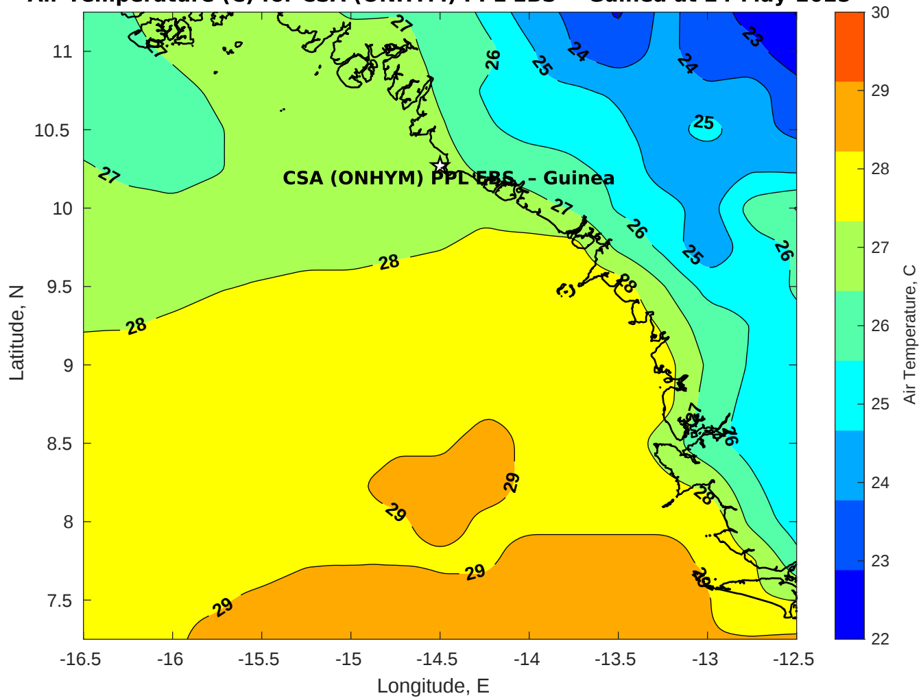
Air Temperature (C) for CSA (ONHYM) PPL EBS - Guinea at 24-May-2025
