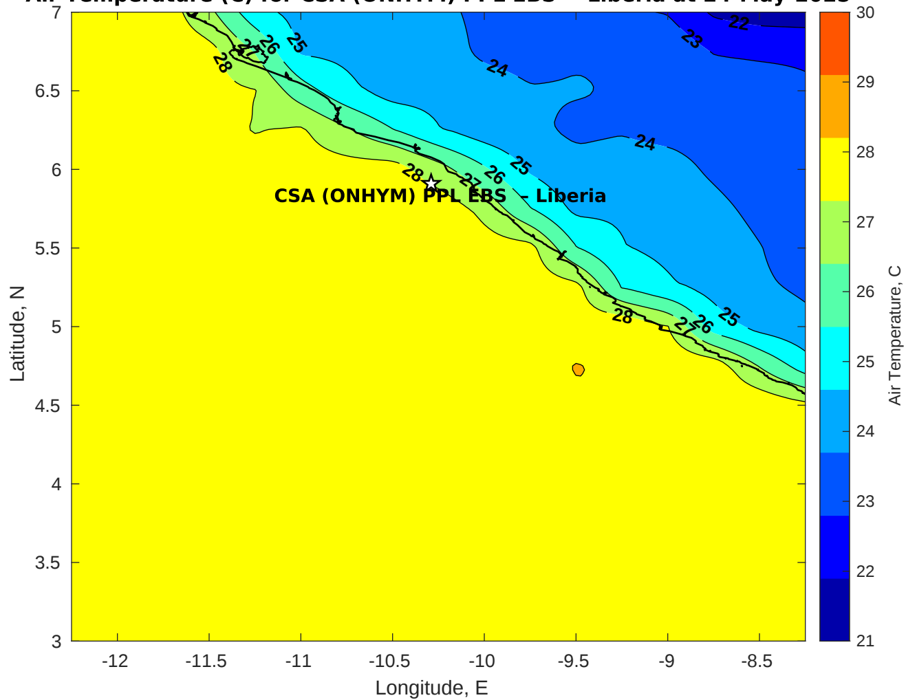
Air Temperature (C) for CSA (ONHYM) PPL EBS - Liberia at 24-May-2025
