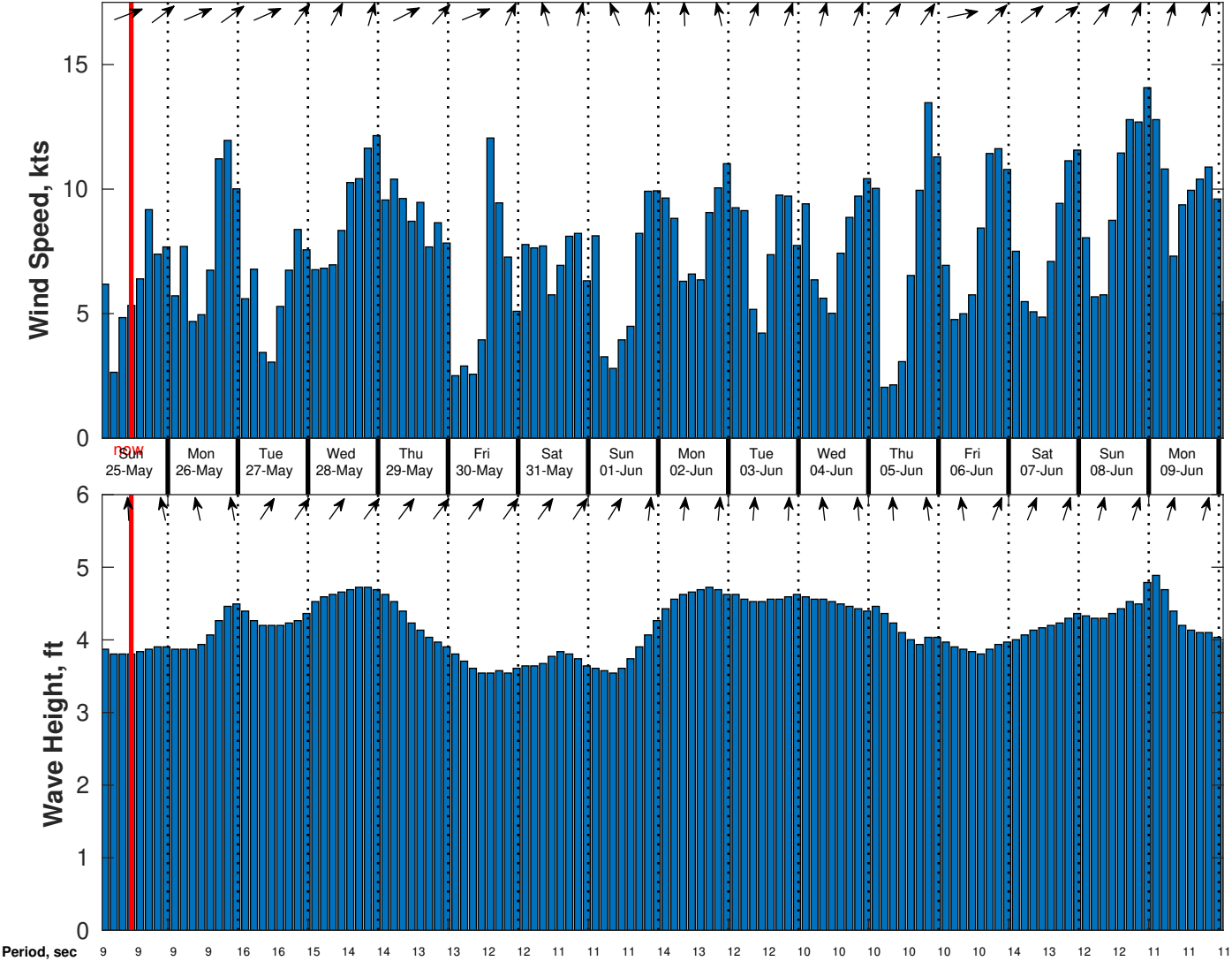
Wind & Wave Forecast for CSA (ONHYM) PPL EBS - Liberia from 24-May-2025 01:00:00 to 09-Jun-2025 01:00:00
