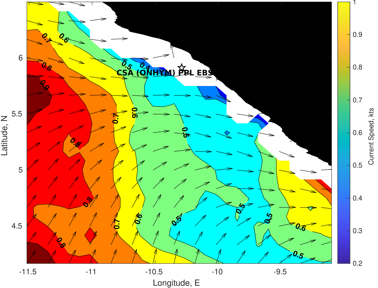
Surface Currents for CSA (ONHYM) PPL EBS - Liberia at 23-May-2025 00:00:00
