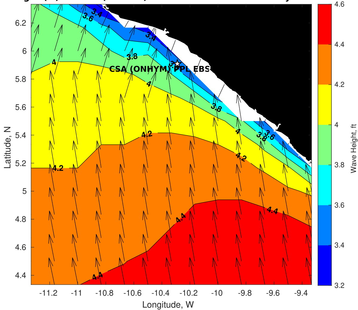
Wave Height (ft) for CSA (ONHYM) PPL EBS - Liberia at 24-May-2025 09:00:00
