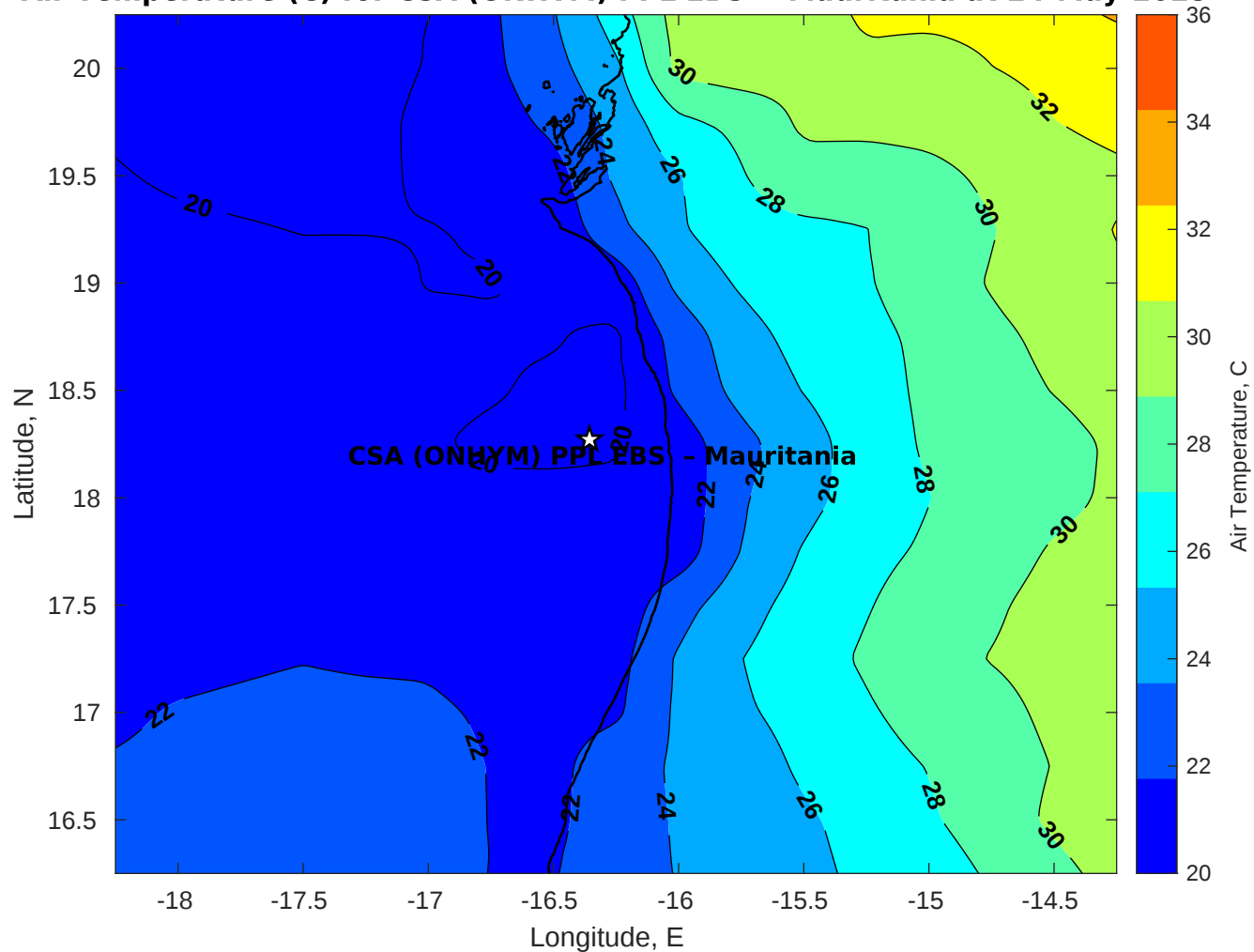
Air Temperature (C) for CSA (ONHYM) PPL EBS - Mauritania at 24-May-2025
