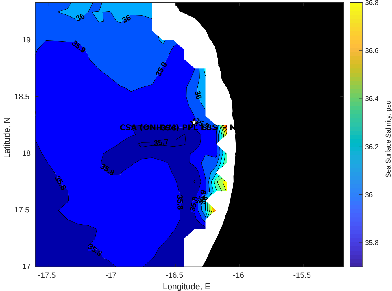
Surface Salinity for CSA (ONHYM) PPL EBS - Mauritania at 23-May-2025 00:00:00
