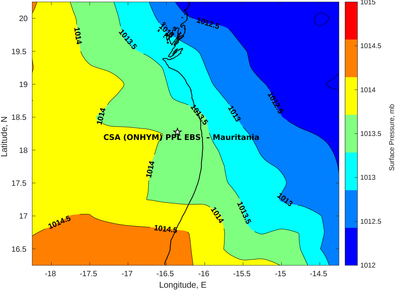
Surface Pressure (mb) for CSA (ONHYM) PPL EBS - Mauritania at 24-May-2025 00:00:00
