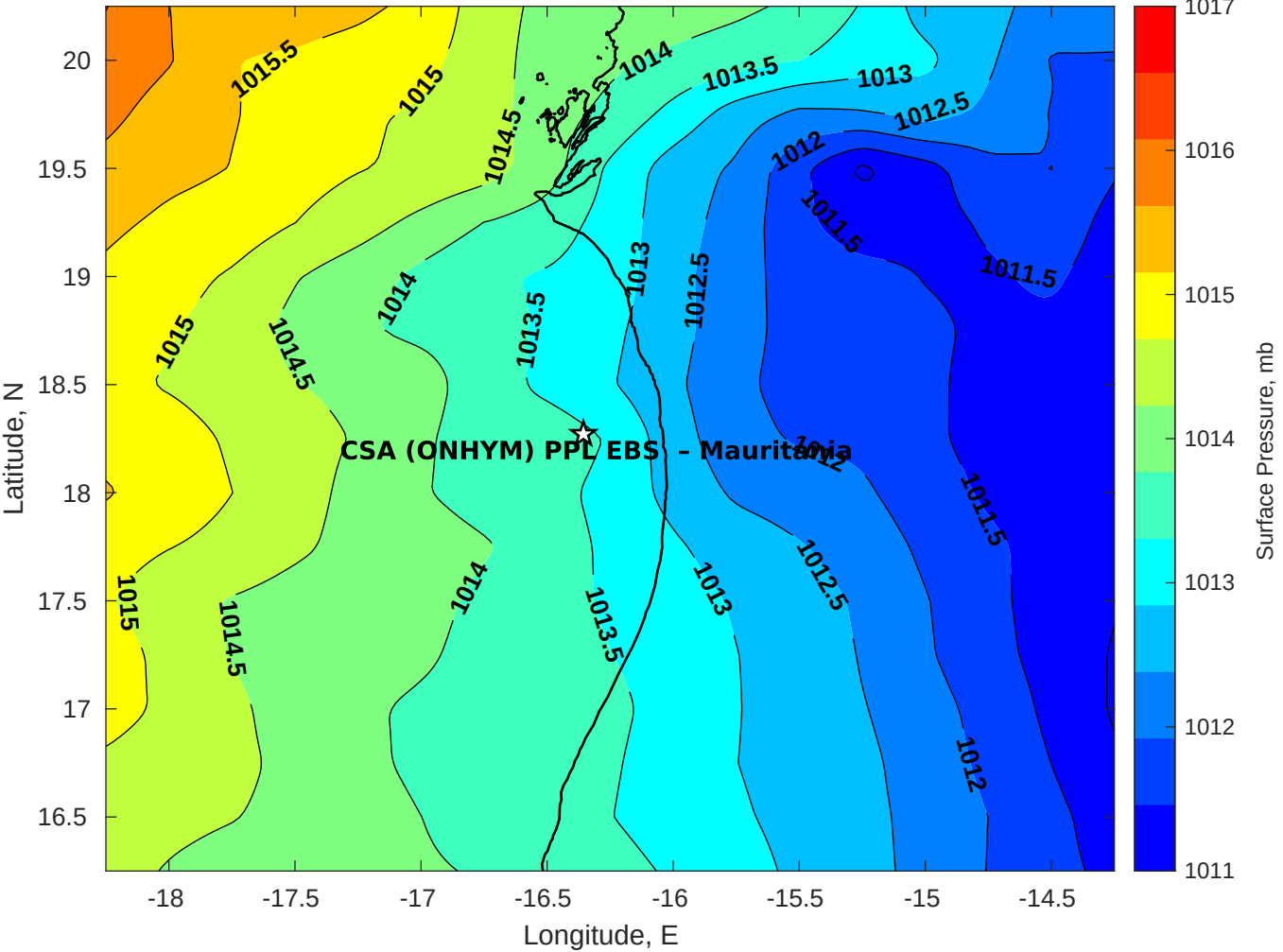
Surface Pressure (mb) for CSA (ONHYM) PPL EBS - Mauritania at 26-May-2025 00:00:00
