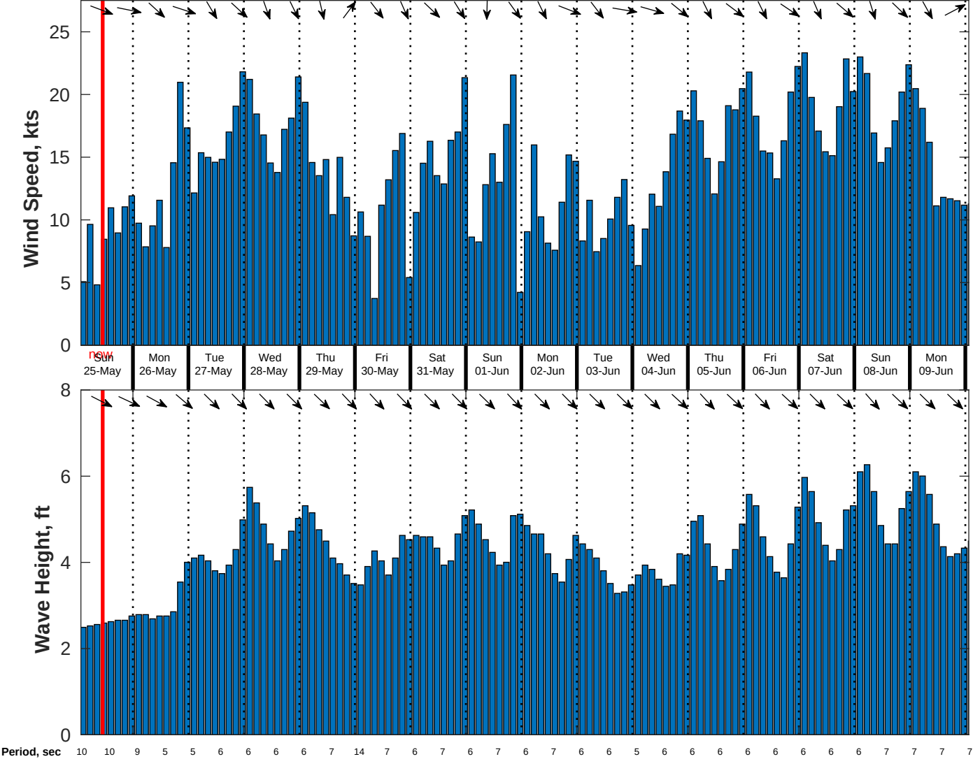
Wind & Wave Forecast for CSA (ONHYM) PPL EBS - Mauritania from 24-May-2025 01:00:00 to 09-Jun-2025 01:00:00
