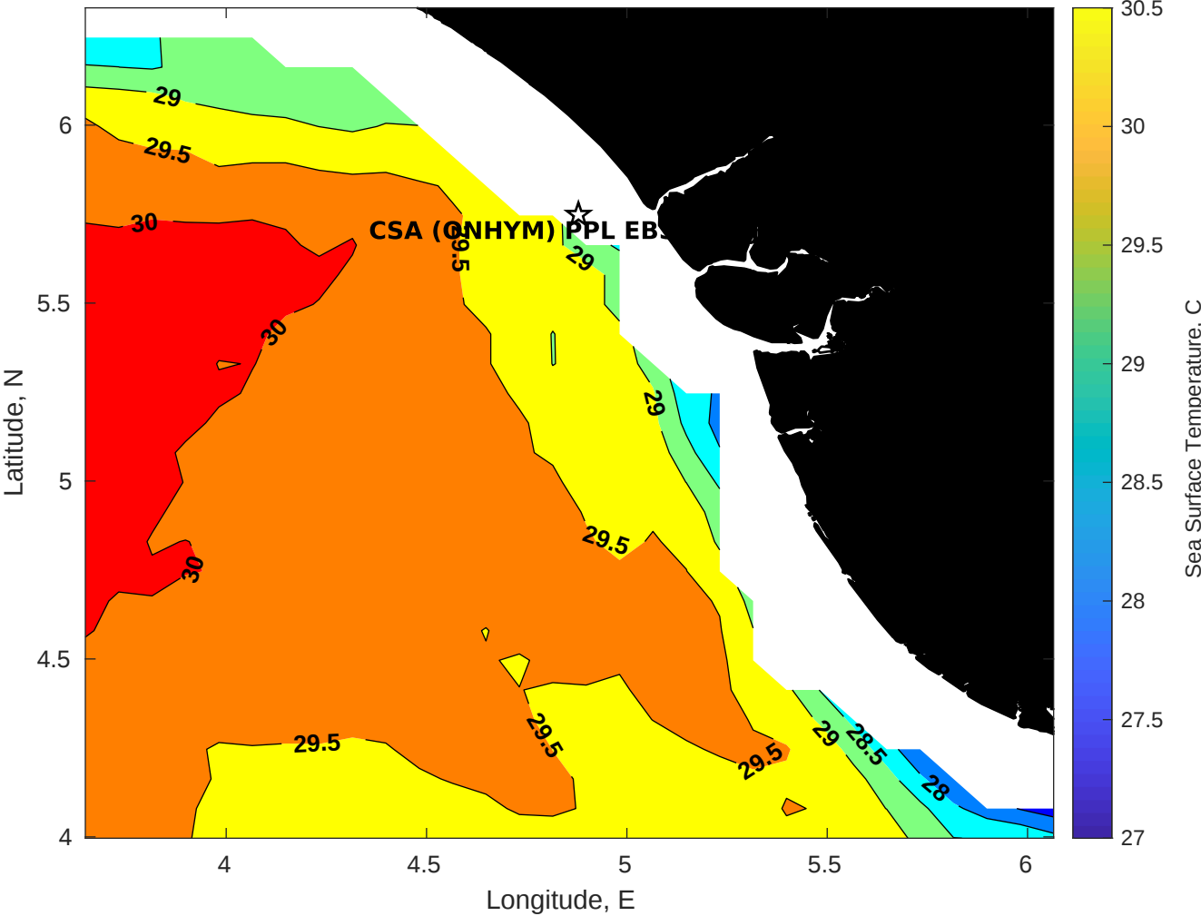
SST for CSA (ONHYM) PPL EBS - Nigeria at 23-May-2025 00:00:00
