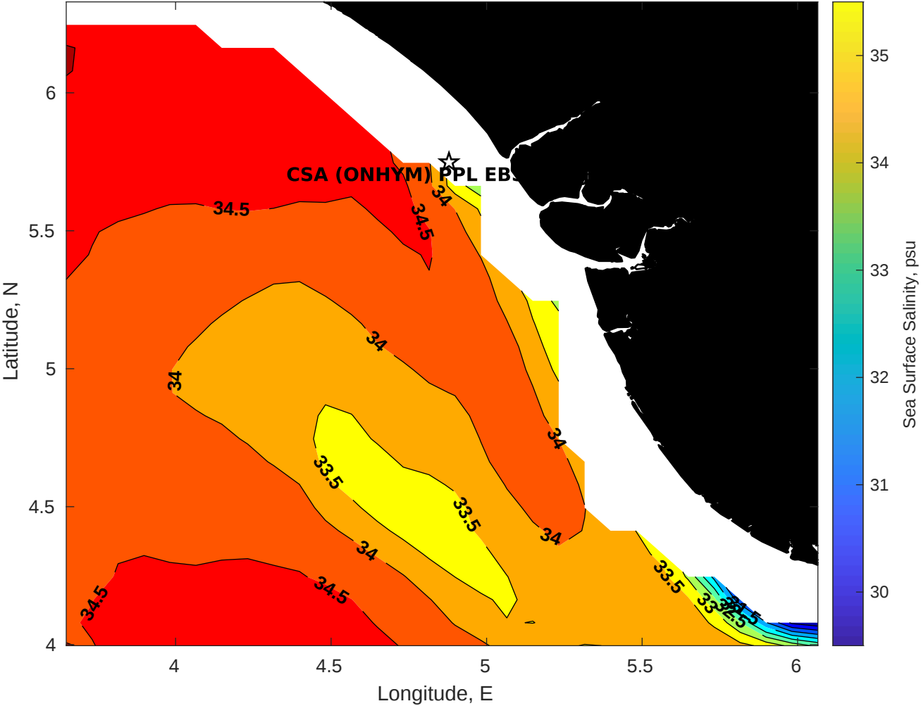
Surface Salinity for CSA (ONHYM) PPL EBS - Nigeria at 23-May-2025 00:00:00
