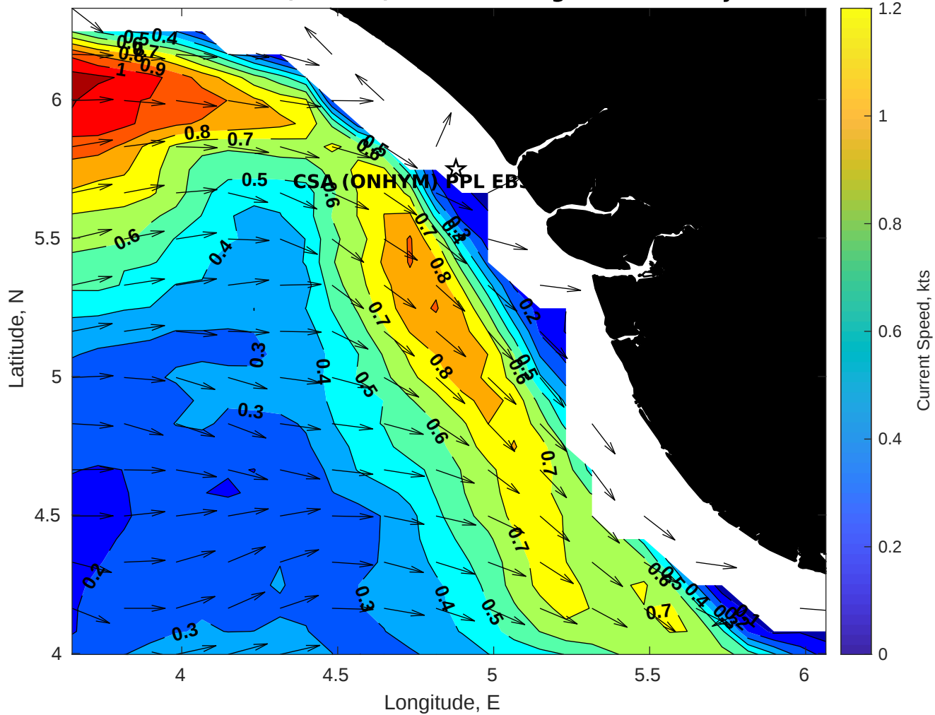
Surface Currents for CSA (ONHYM) PPL EBS - Nigeria at 23-May-2025 00:00:00
