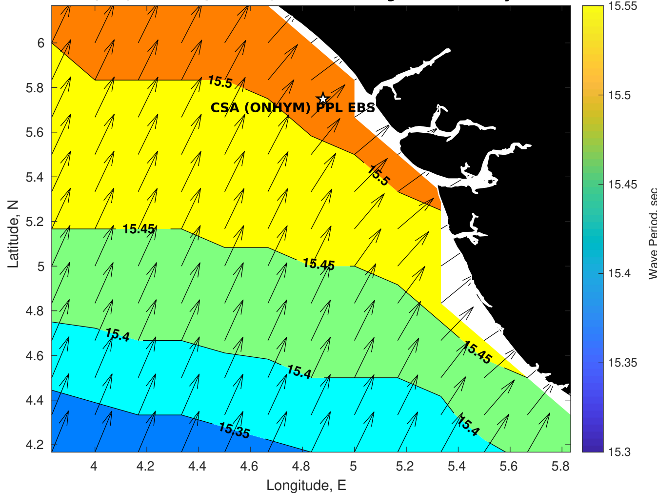
Wave Period (sec) for CSA (ONHYM) PPL EBS - Nigeria at 24-May-2025 09:00:00
