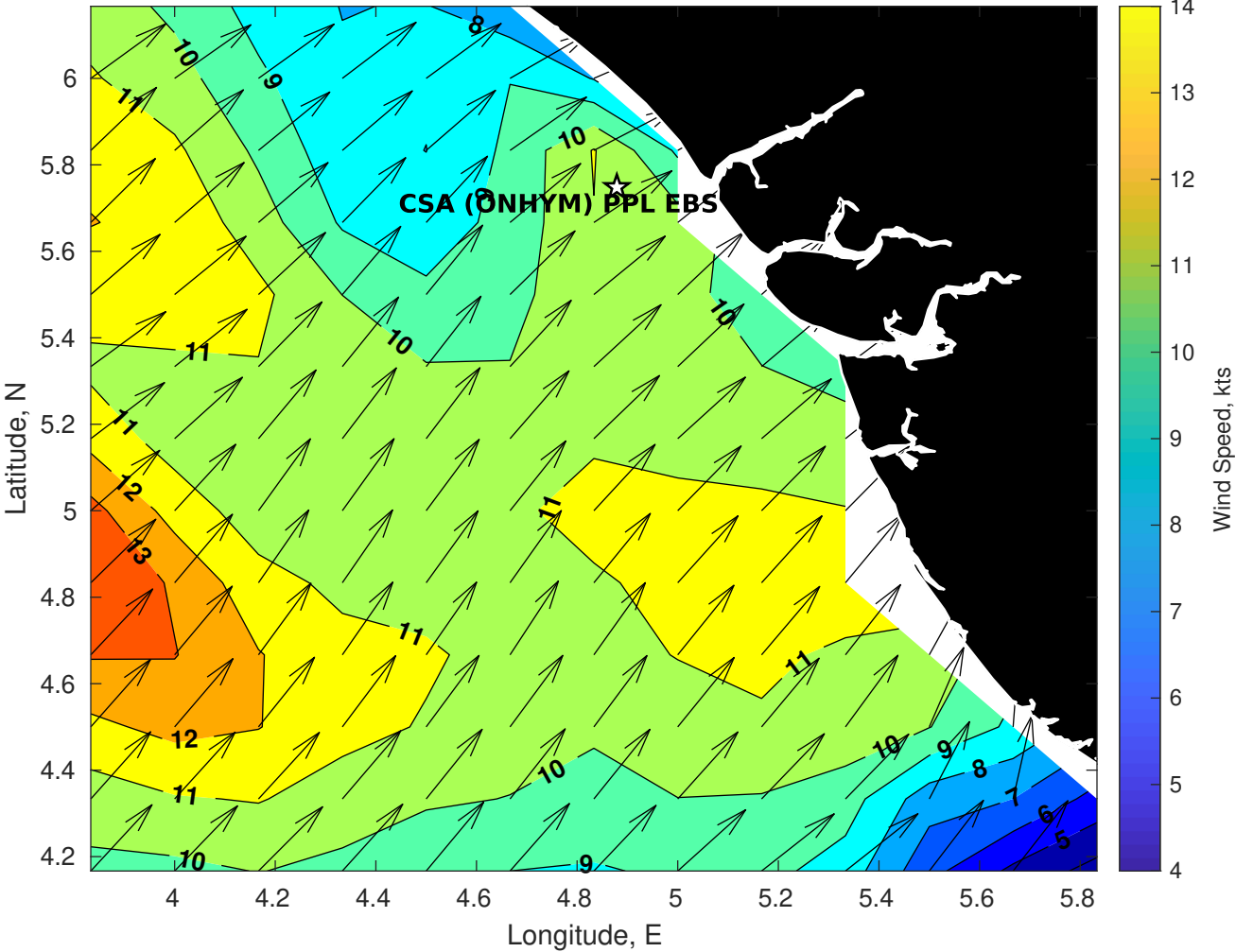
Winds (kts) for CSA (ONHYM) PPL EBS - Nigeria at 24-May-2025 09:00:00
