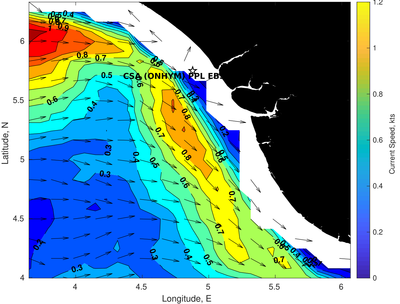
Surface Currents for CSA (ONHYM) PPL EBS - Nigeria at 23-May-2025 00:00:00
