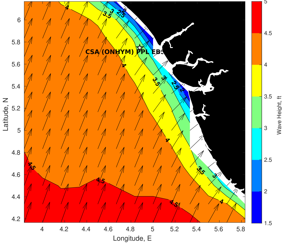
Wave Height (ft) for CSA (ONHYM) PPL EBS - Nigeria at 24-May-2025 09:00:00
