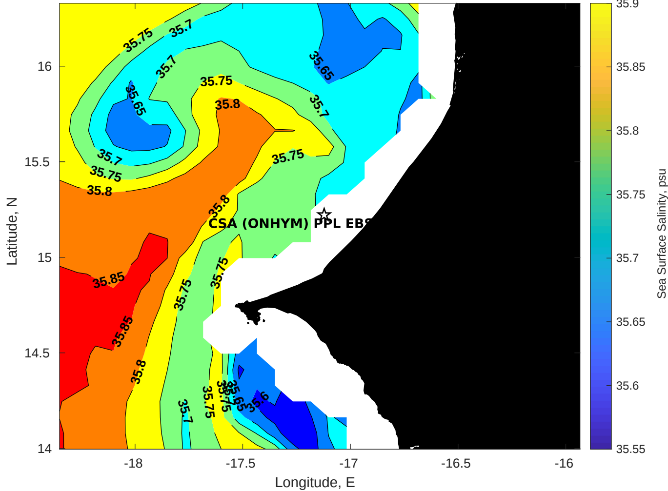
Surface Salinity for CSA (ONHYM) PPL EBS - Senegal at 23-May-2025 00:00:00
