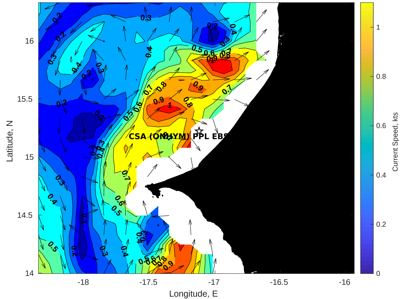
Surface Currents for CSA (ONHYM) PPL EBS - Senegal at 23-May-2025 00:00:00
