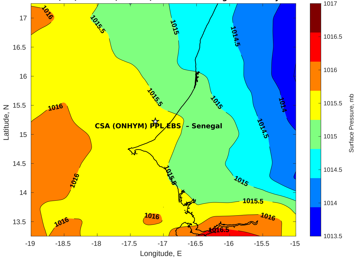
Surface Pressure (mb) for CSA (ONHYM) PPL EBS - Senegal at 25-May-2025 00:00:00
