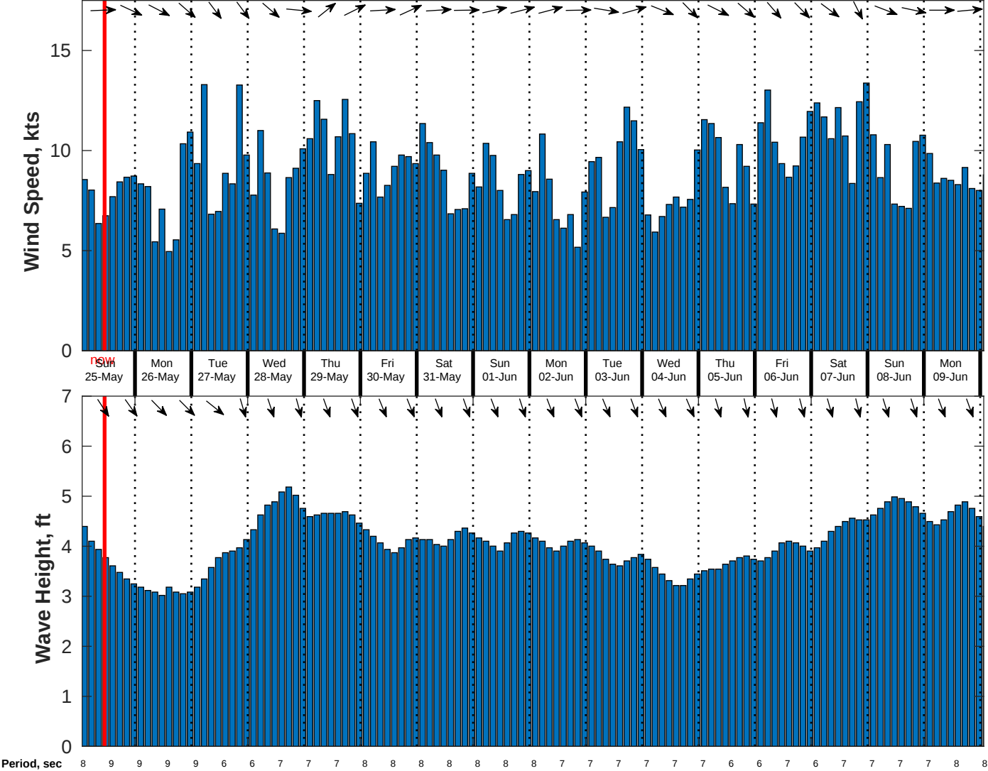
Wind & Wave Forecast for CSA (ONHYM) PPL EBS - Senegal from 24-May-2025 01:00:00 to 09-Jun-2025 01:00:00
