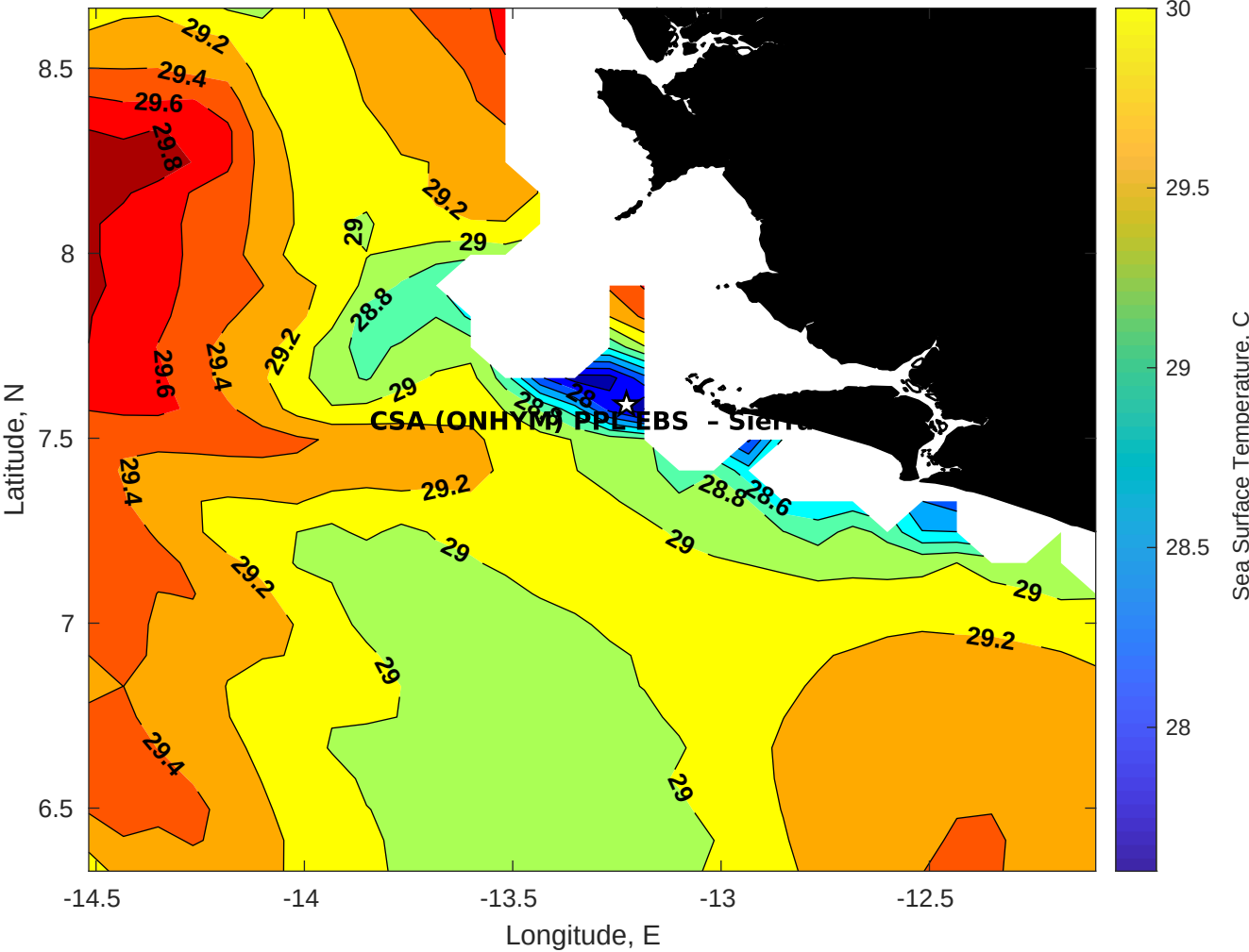
SST for CSA (ONHYM) PPL EBS - Sierra Leone at 23-May-2025 00:00:00
