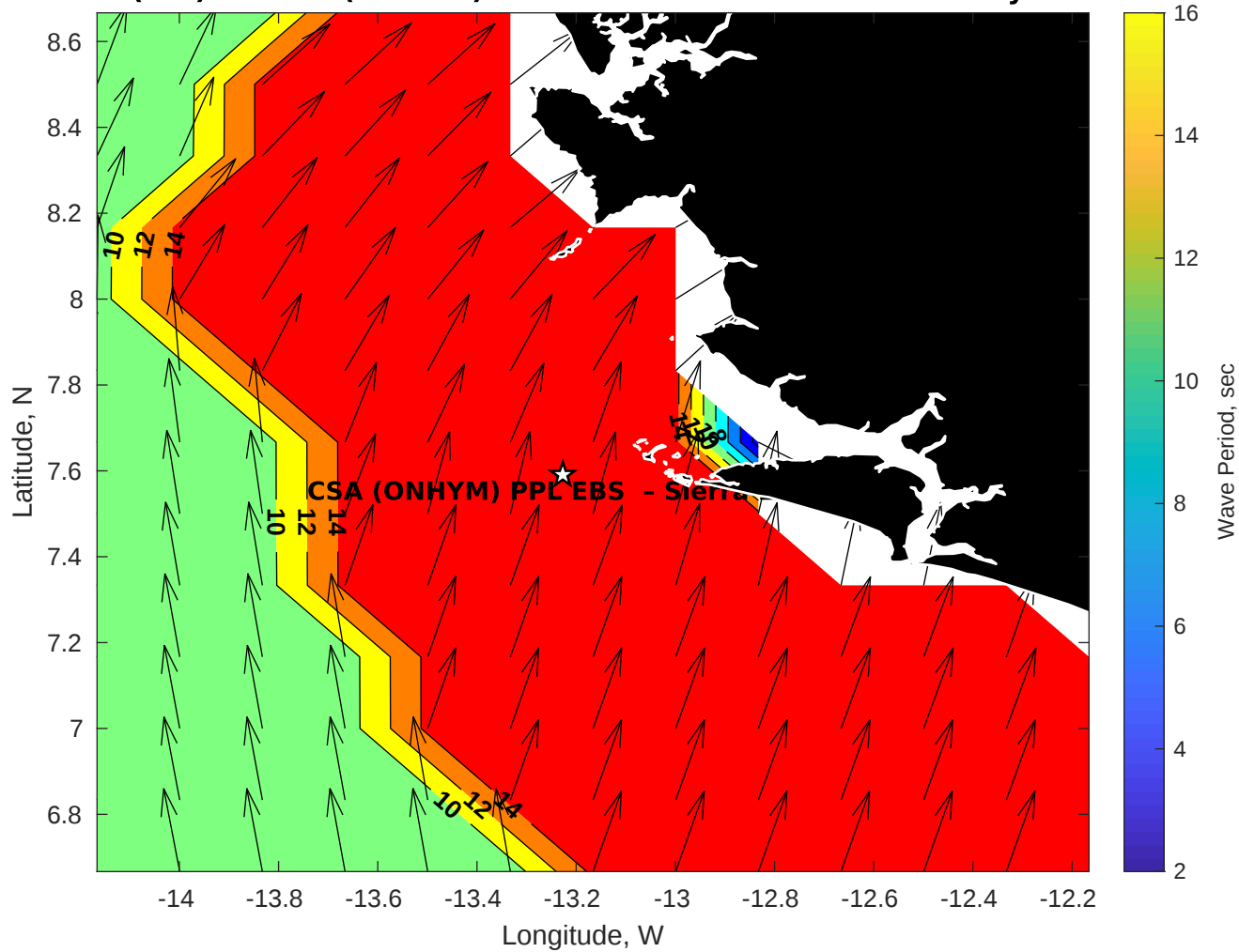
Wave Period (sec) for CSA (ONHYM) PPL EBS - Sierra Leone at 24-May-2025 09:00:00
