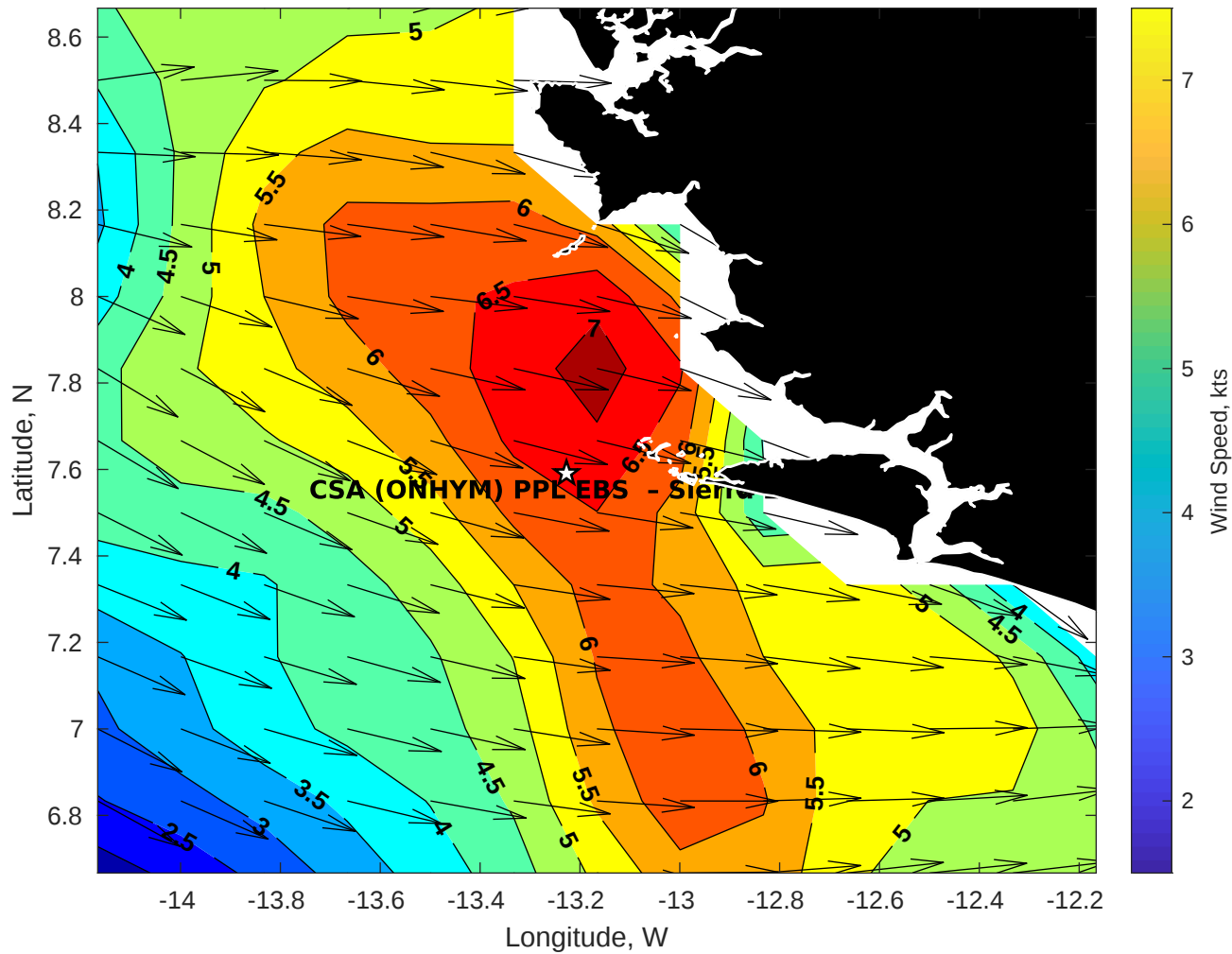
Winds (kts) for CSA (ONHYM) PPL EBS - Sierra Leone at 24-May-2025 09:00:00
