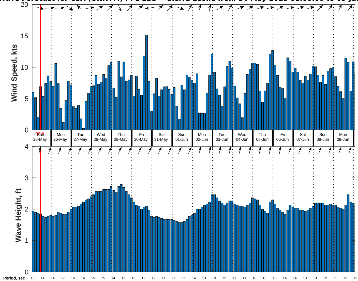
Wind & Wave Forecast for CSA (ONHYM) PPL EBS - Sierra Leone from 24-May-2025 01:00:00 to 09-Jun-2025 01:00:00
