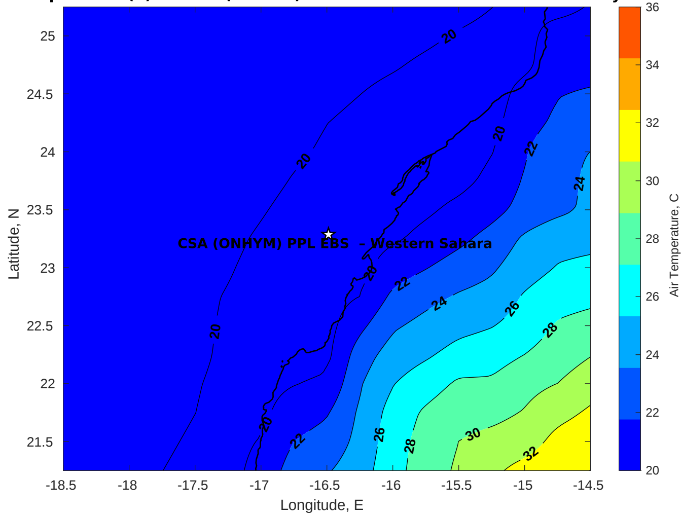
Air Temperature (C) for CSA (ONHYM) PPL EBS - Western Sahara at 24-May-2025
