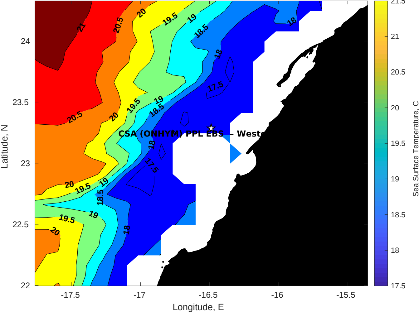
SST for CSA (ONHYM) PPL EBS - Western Sahara at 23-May-2025 00:00:00
