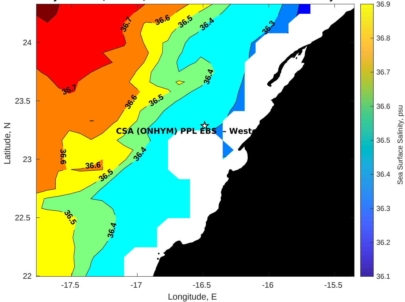
Surface Salinity for CSA (ONHYM) PPL EBS - Western Sahara at 23-May-2025 00:00:00
