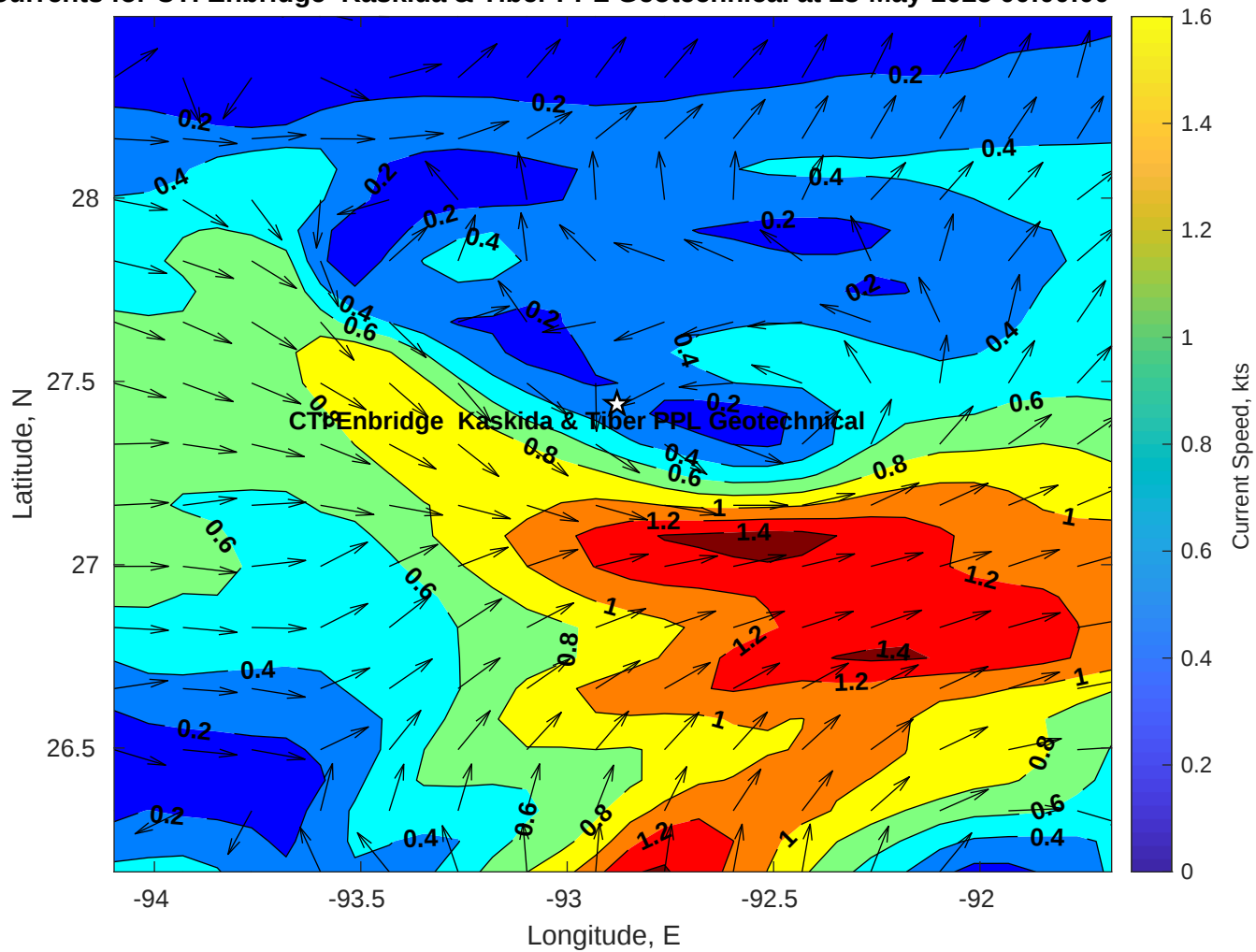
Surface Currents for CTI Enbridge Kaskida & Tiber PPL Geotechnical at 23-May-2025 00:00:00
