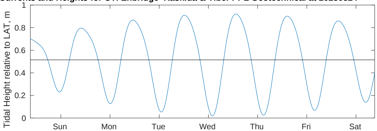
Tidal Currents and Heights for CTI Enbridge Kaskida & Tiber PPL Geotechnical at 20250524
