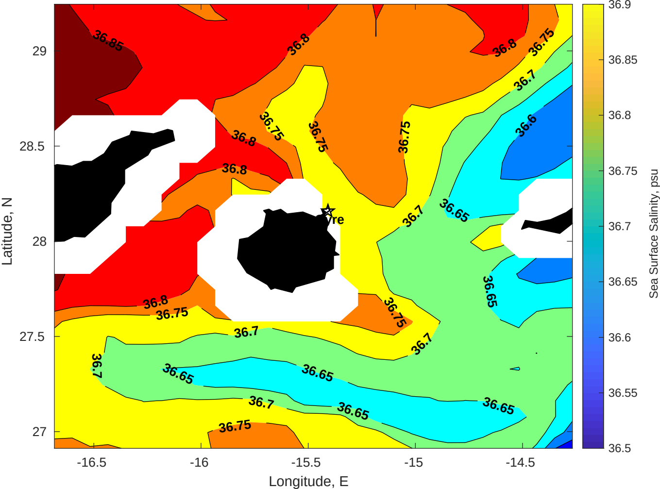
Surface Salinity for Gyre at 23-May-2025 00:00:00
