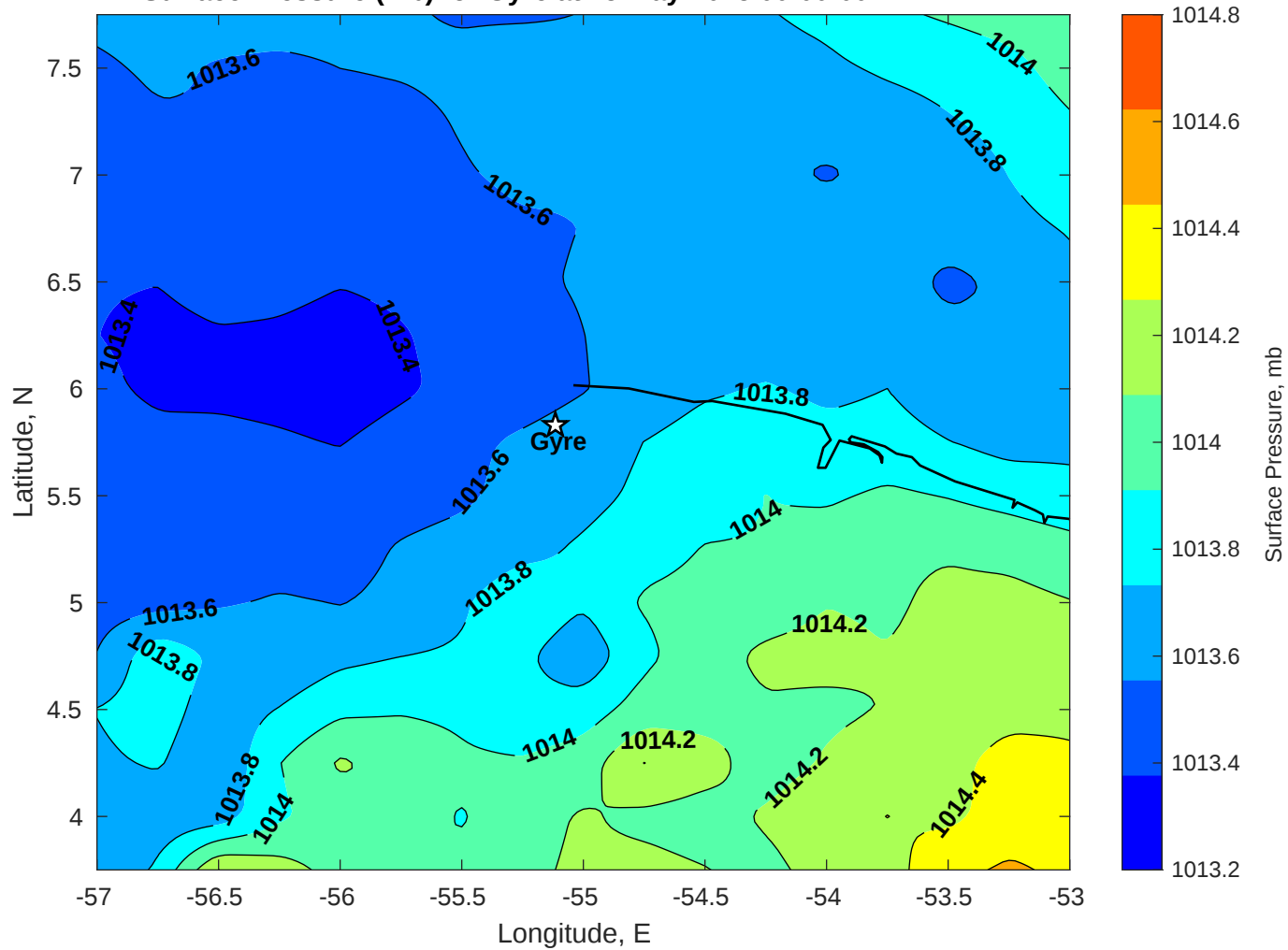
Surface Pressure (mb) for Gyre at 25-May-2025 00:00:00
