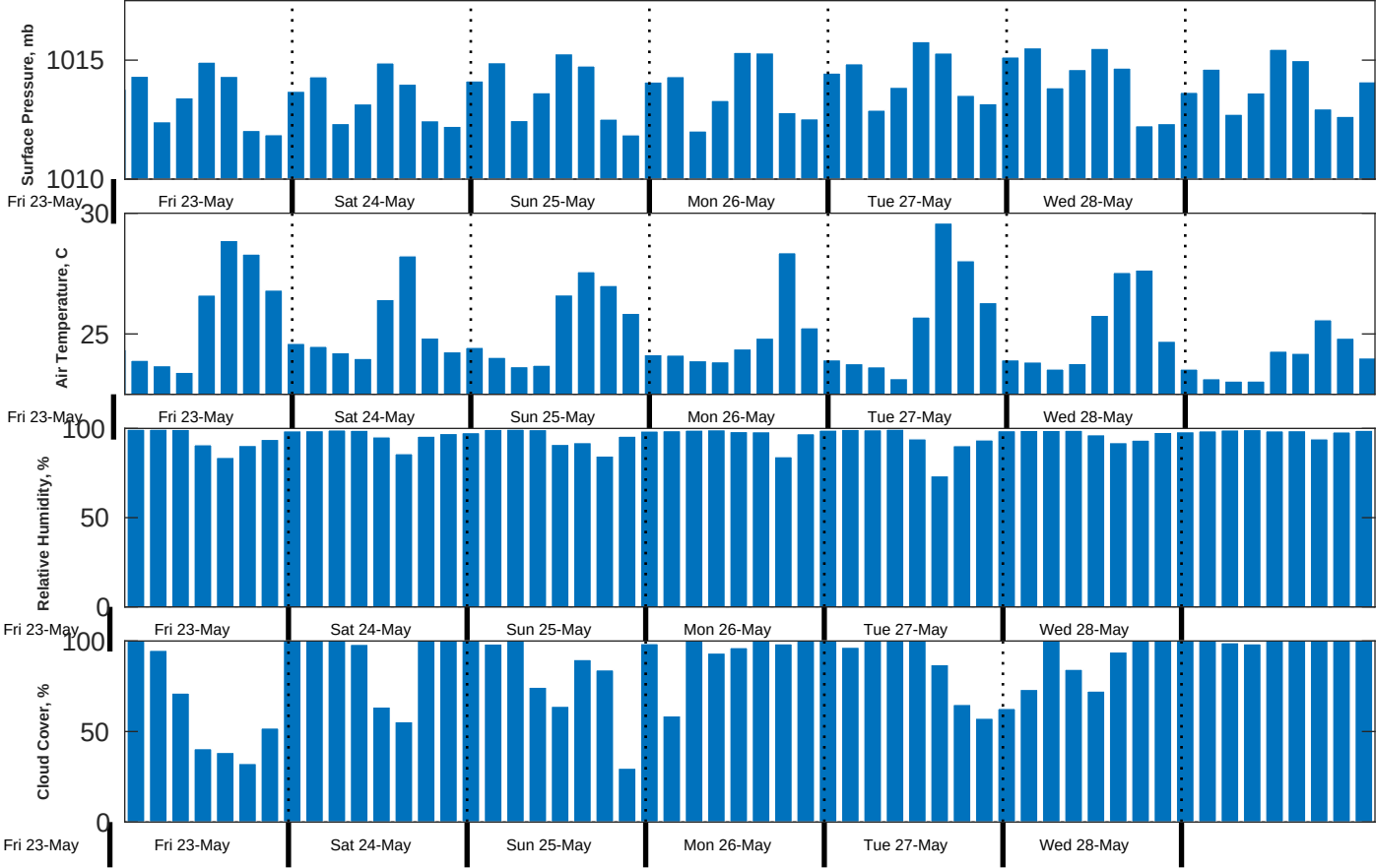
Met Forecast for Gyre from 23-May-2025 20:00:00 to 30-May-2025 20:00:00
