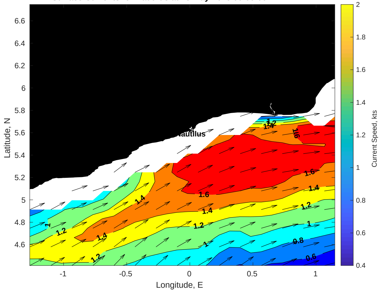
Surface Currents for Nautilus at 23-May-2025 00:00:00
