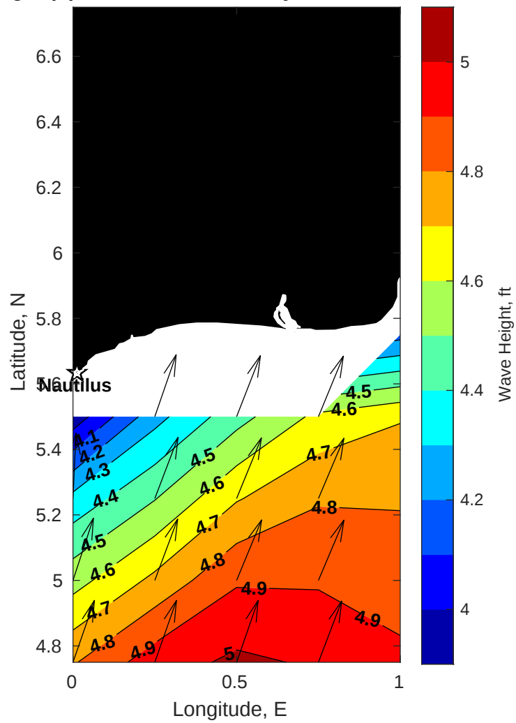
Wave Height (ft) for Nautilus at 24-May-2025 09:00:00
