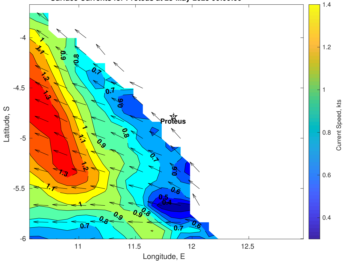
Surface Currents for Proteus at 23-May-2025 00:00:00
