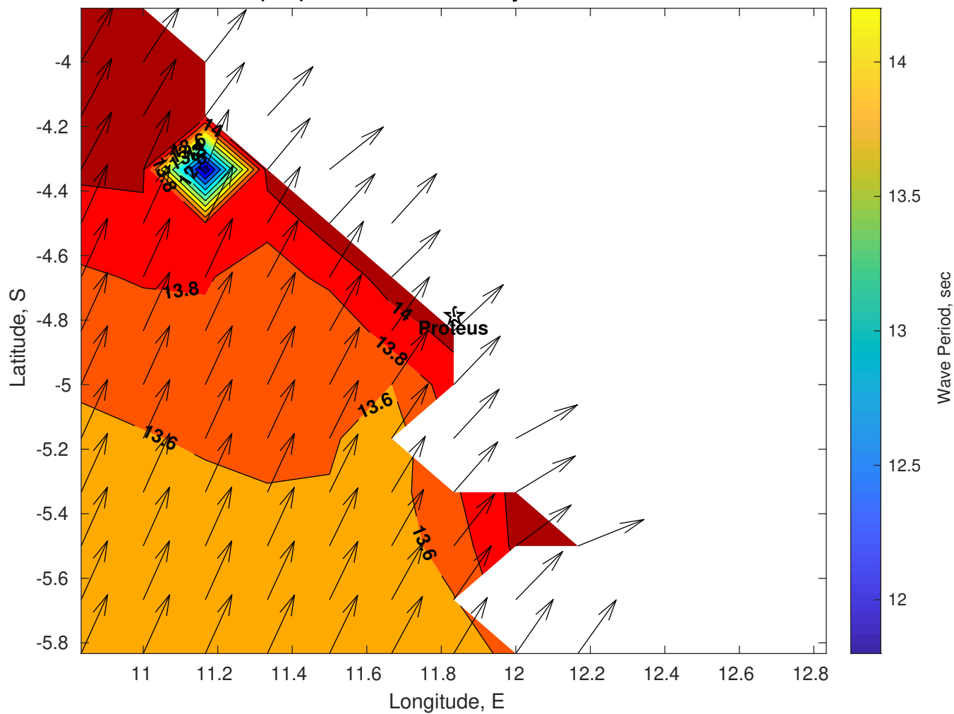
Wave Period (sec) for Proteus at 24-May-2025 09:00:00
