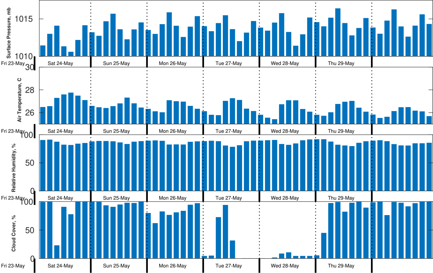
Met Forecast for Proteus from 24-May-2025 00:00:00 to 31-May-2025 00:00:00
