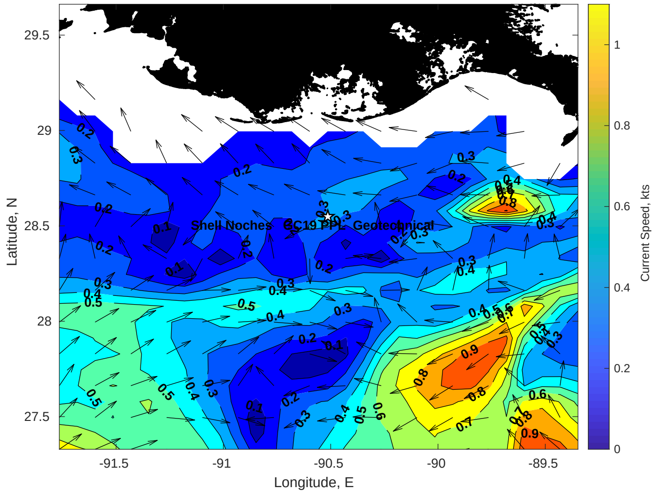
Surface Currents for Shell Noches GC19 PPL Geotechnical at 23-May-2025 00:00:00
