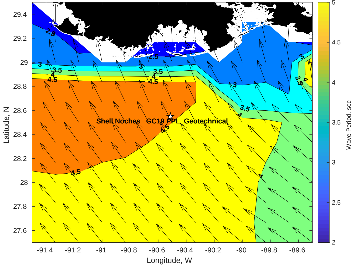
Wave Period (sec) for Shell Noches GC19 PPL Geotechnical at 24-May-2025 09:00:00
