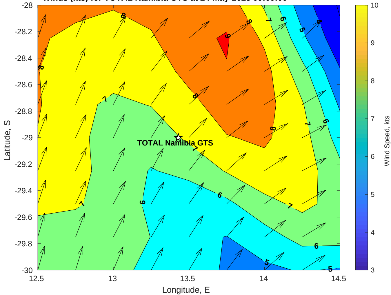
Winds (kts) for TOTAL Namibia GTS at 24-May-2025 09:00:00
