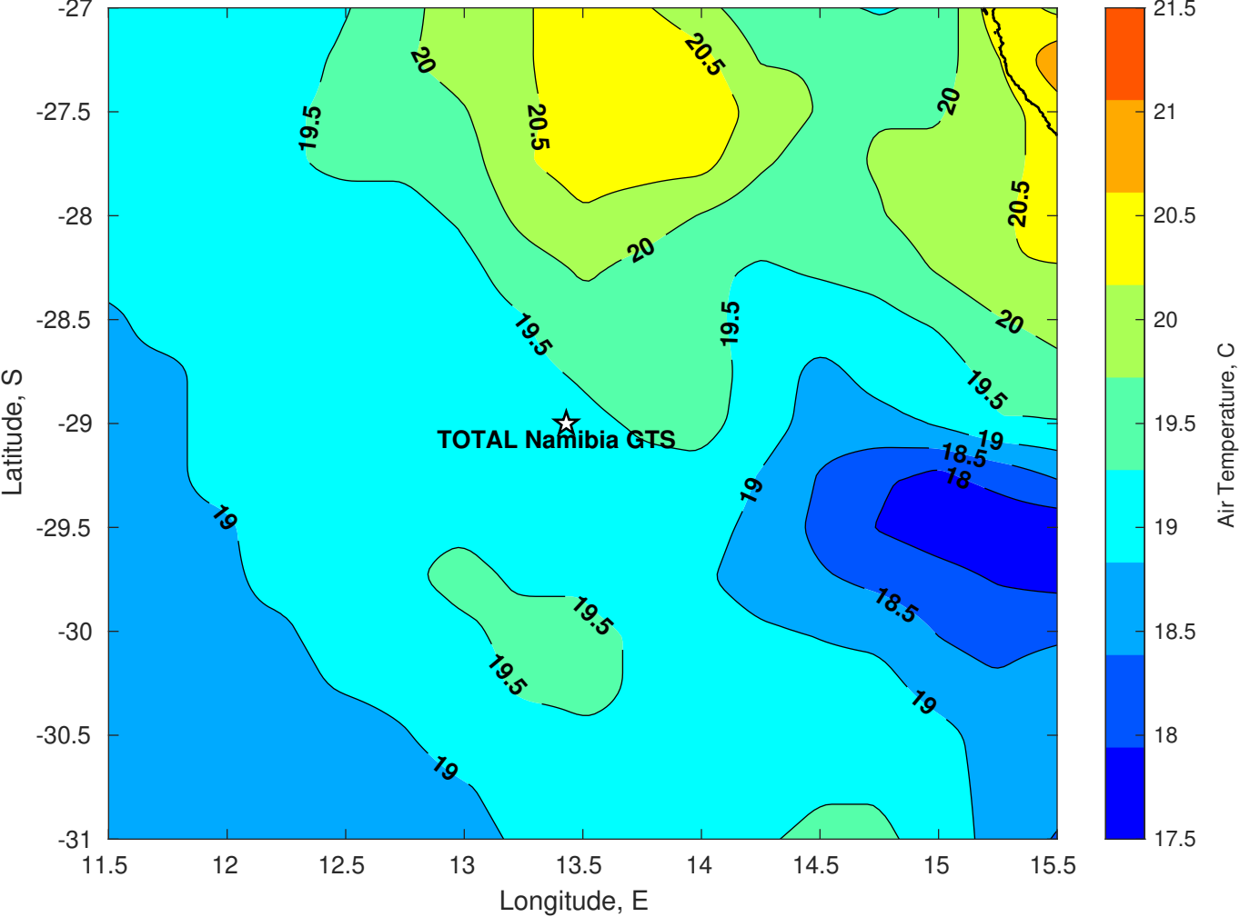
Air Temperature (C) for TOTAL Namibia GTS at 24-May-2025
