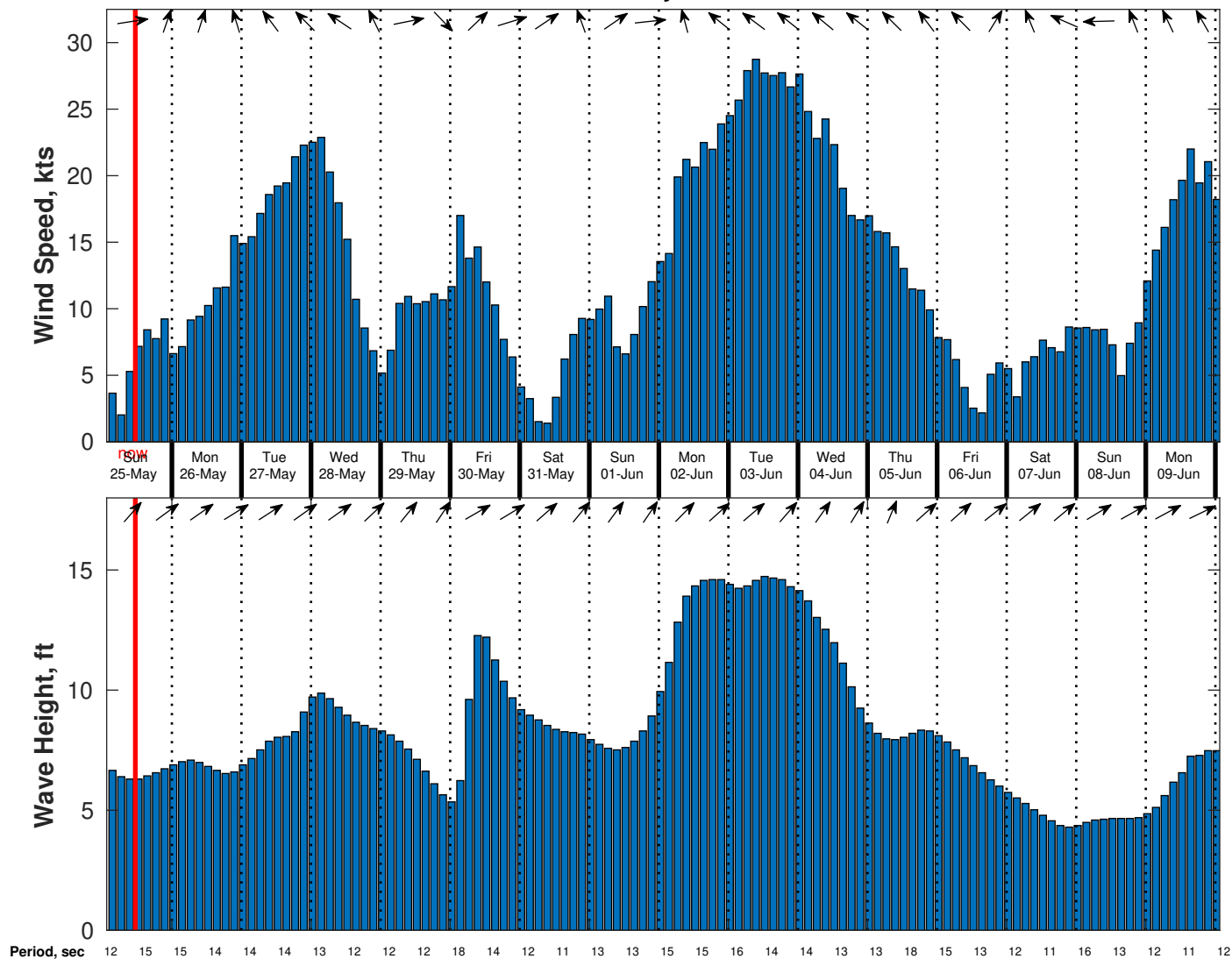
Wind & Wave Forecast for TOTAL Namibia GTS from 24-May-2025 02:00:00 to 09-Jun-2025 02:00:00
