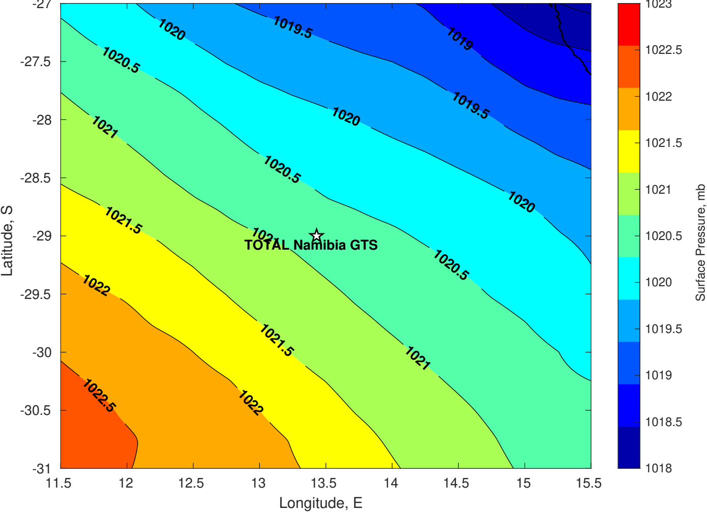
Surface Pressure (mb) for TOTAL Namibia GTS at 26-May-2025 00:00:00
