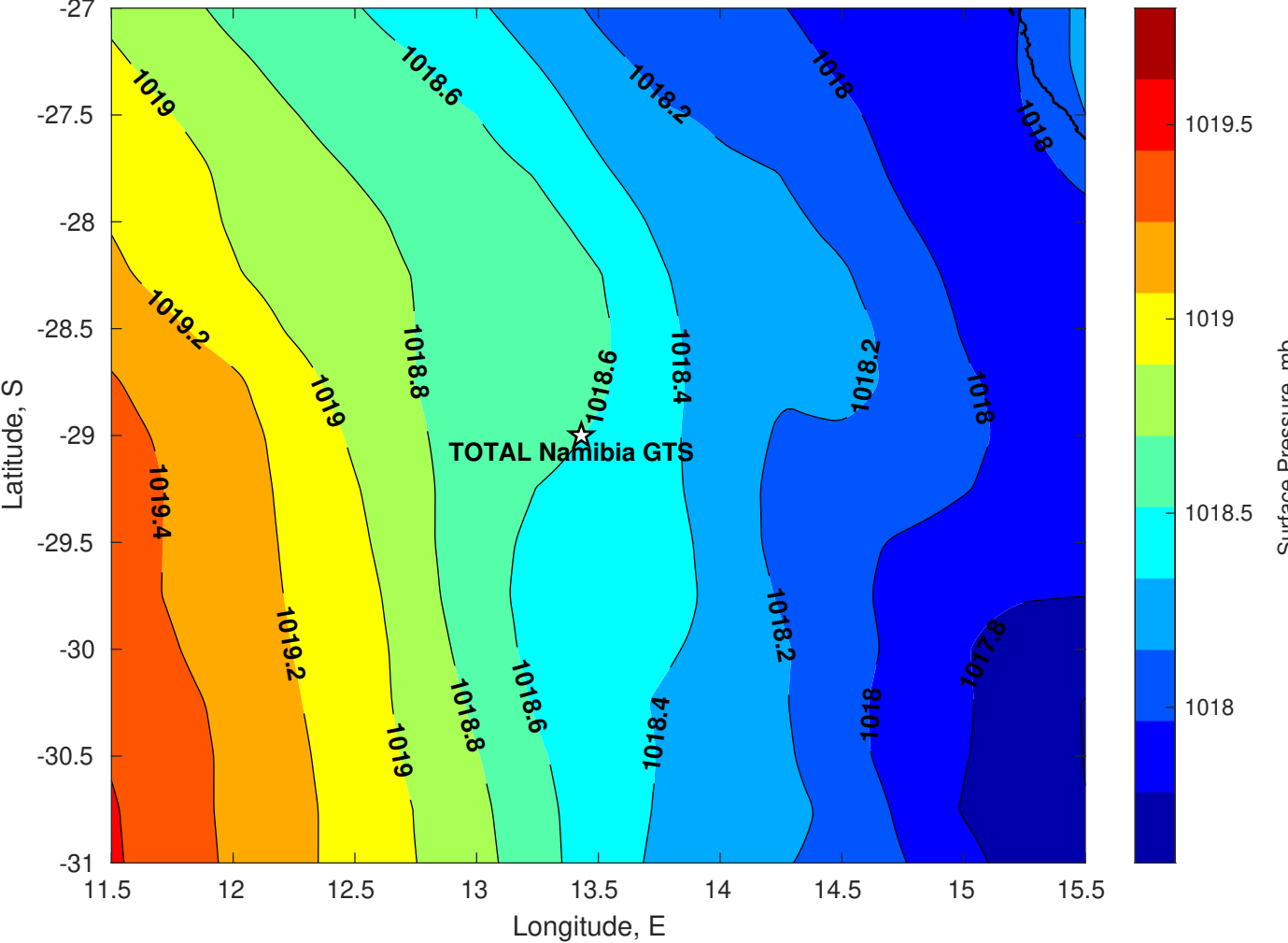
Surface Pressure (mb) for TOTAL Namibia GTS at 25-May-2025 00:00:00
