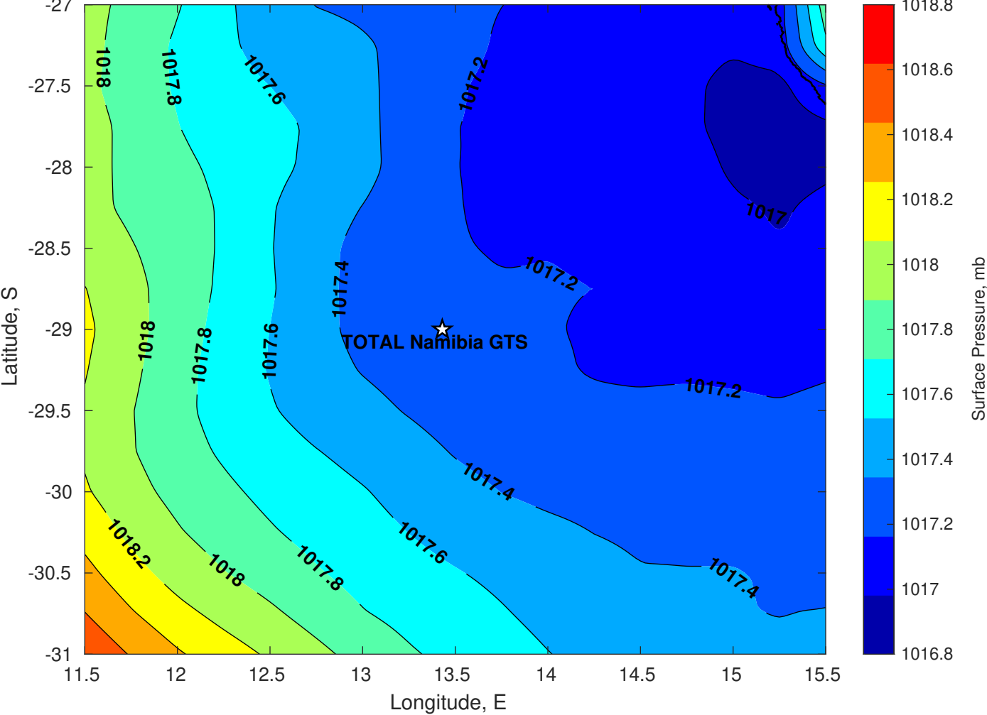
Surface Pressure (mb) for TOTAL Namibia GTS at 24-May-2025 00:00:00
