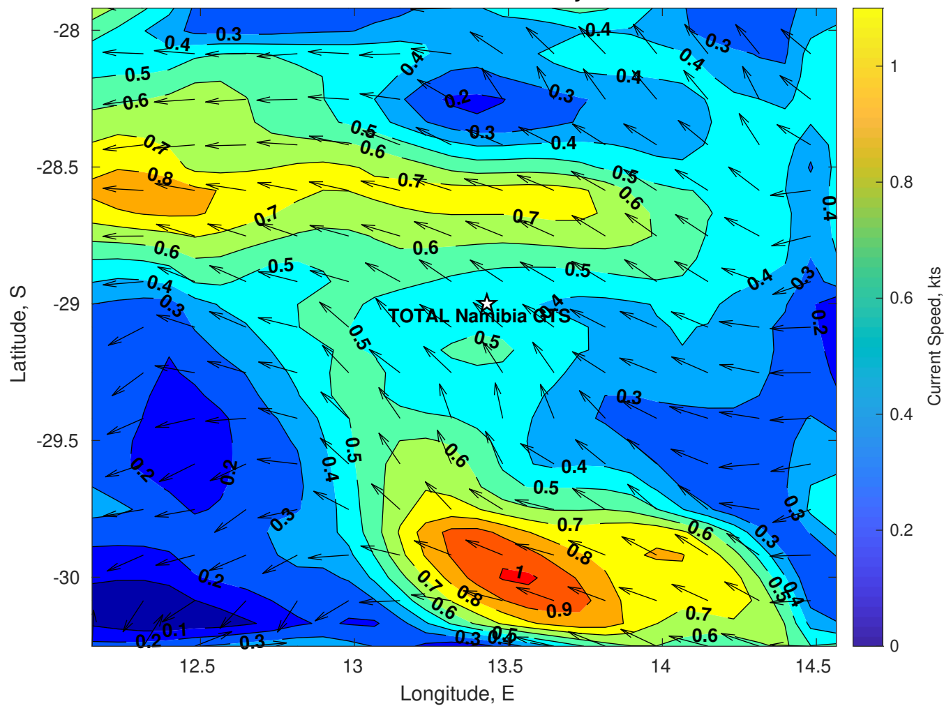
Surface Currents for TOTAL Namibia GTS at 23-May-2025 00:00:00
