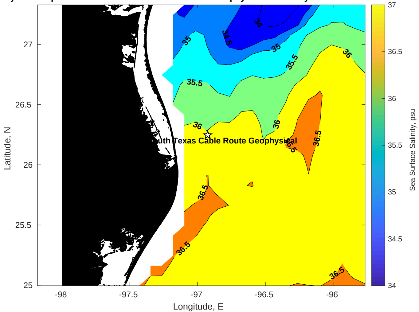
Surface Salinity for Tampnet P2378 South Texas Cable Route Geophysical at 23-May-2025 00:00:00
