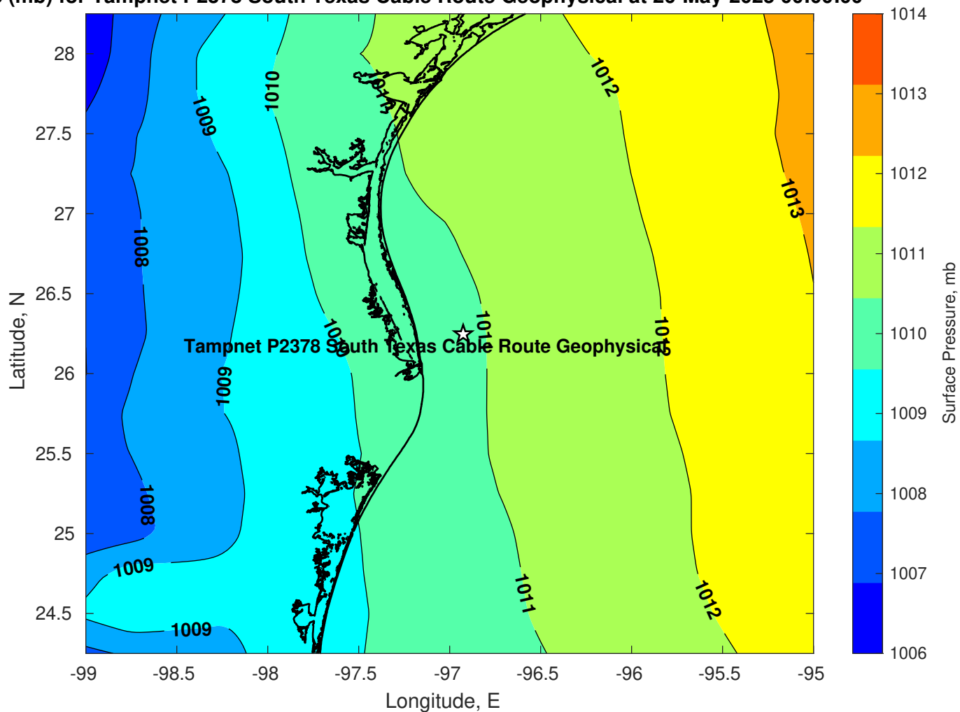
Pressure (mb) for Tampnet P2378 South Texas Cable Route Geophysical at 26-May-2025 00:00:00
