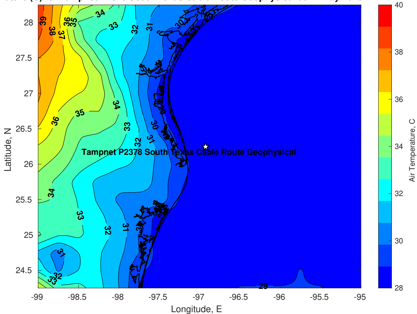
Air Temperature (C) for Tampnet P2378 South Texas Cable Route Geophysical at 24-May-2025
