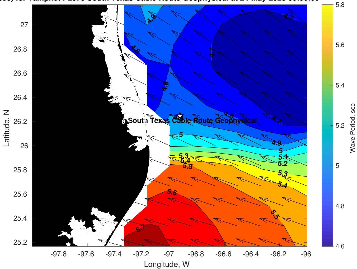
Period (sec) for Tampnet P2378 South Texas Cable Route Geophysical at 24-May-2025 09:00:00
