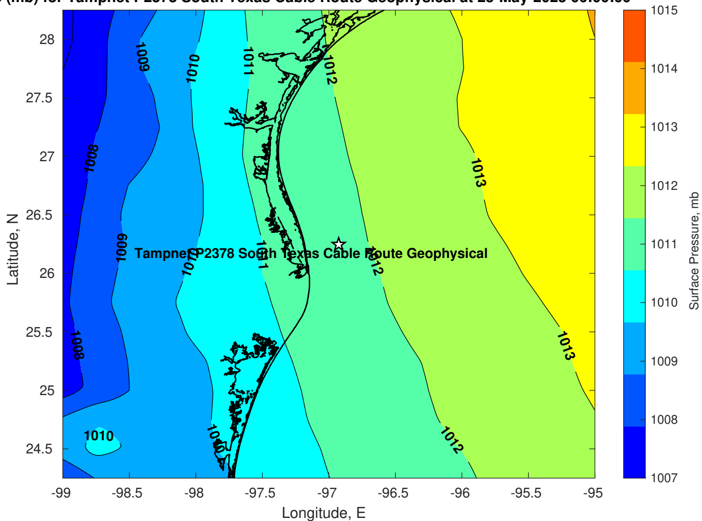
Pressure (mb) for Tampnet P2378 South Texas Cable Route Geophysical at 25-May-2025 00:00:00
