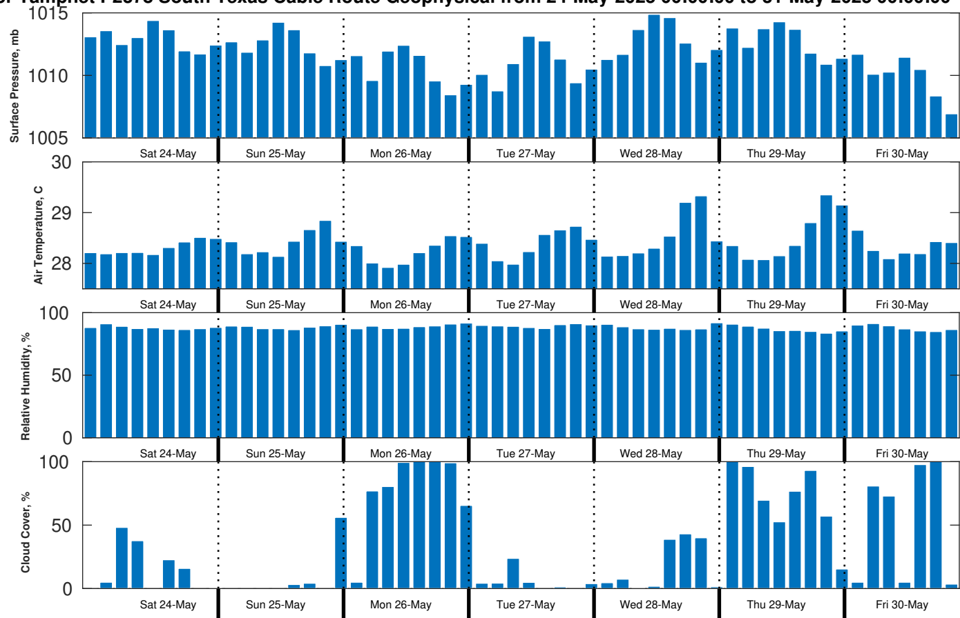
Met Forecast for Tampnet P2378 South Texas Cable Route Geophysical from 24-May-2025 00:00:00 to 31-May-2025 00:00:00
