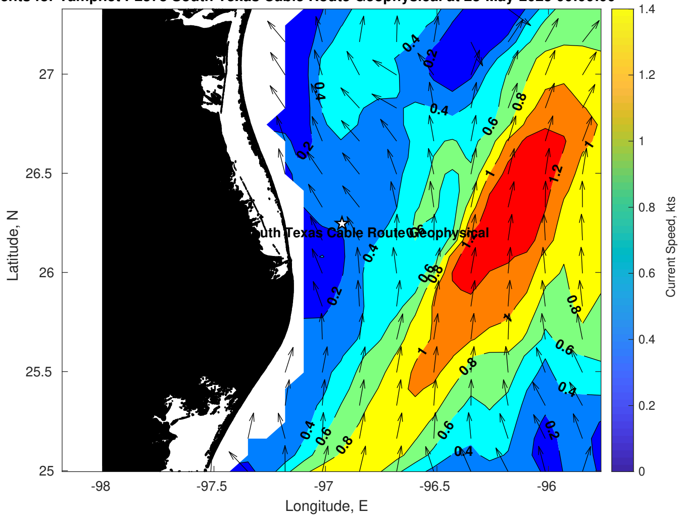
Surface Currents for Tampnet P2378 South Texas Cable Route Geophysical at 23-May-2025 00:00:00
