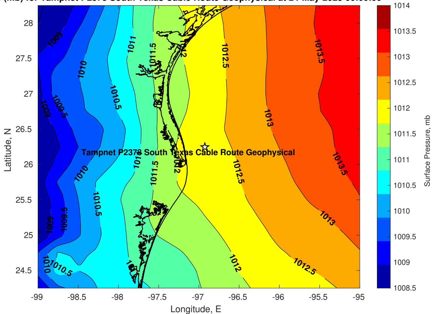
Pressure (mb) for Tampnet P2378 South Texas Cable Route Geophysical at 24-May-2025 00:00:00
