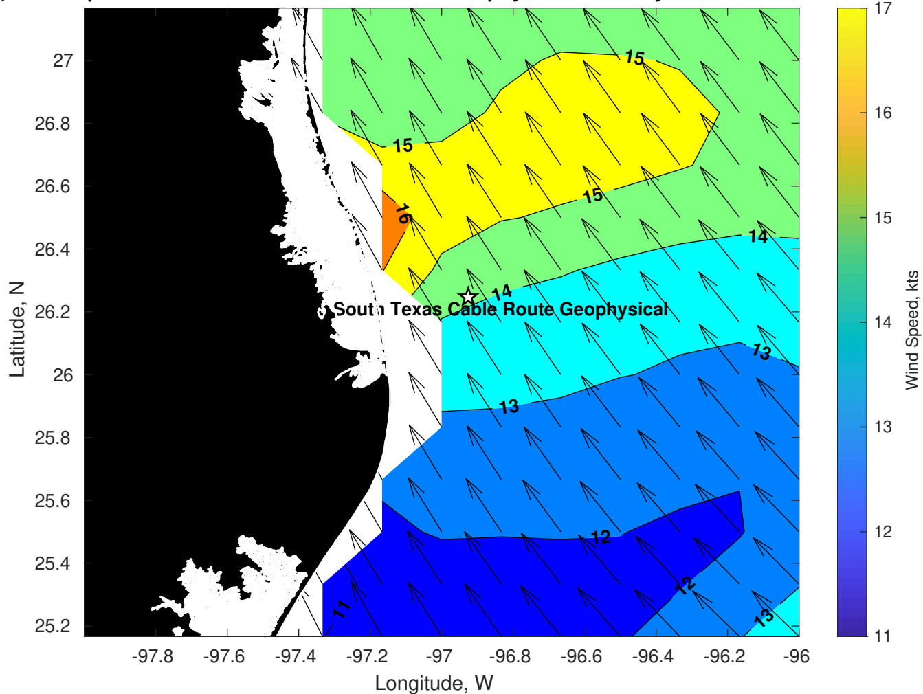
Winds (kts) for Tampnet P2378 South Texas Cable Route Geophysical at 24-May-2025 09:00:00
