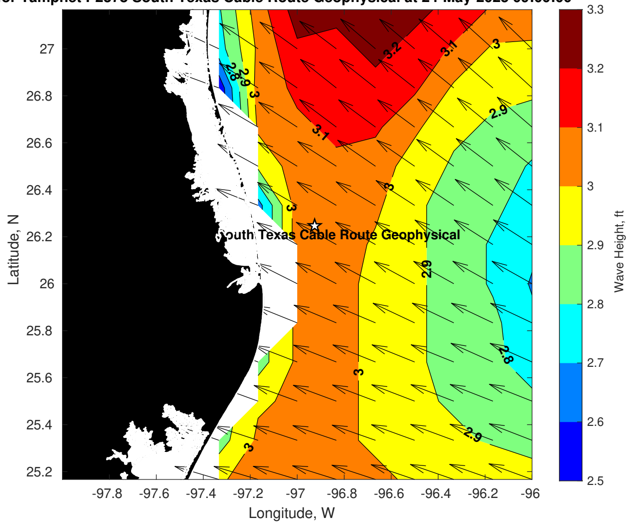
Wave Height (ft) for Tampnet P2378 South Texas Cable Route Geophysical at 24-May-2025 09:00:00
