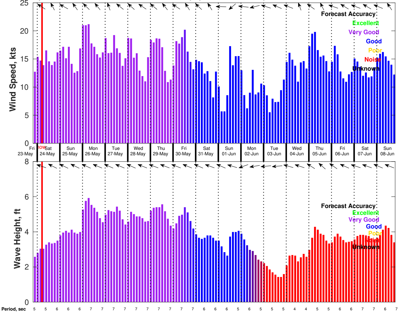
Wind & Wave Forecast for Tampnet P2378 South Texas Cable Route Geophysical from 23-May-2025 20:00:00 to 08-Jun-2025 20:00:00
