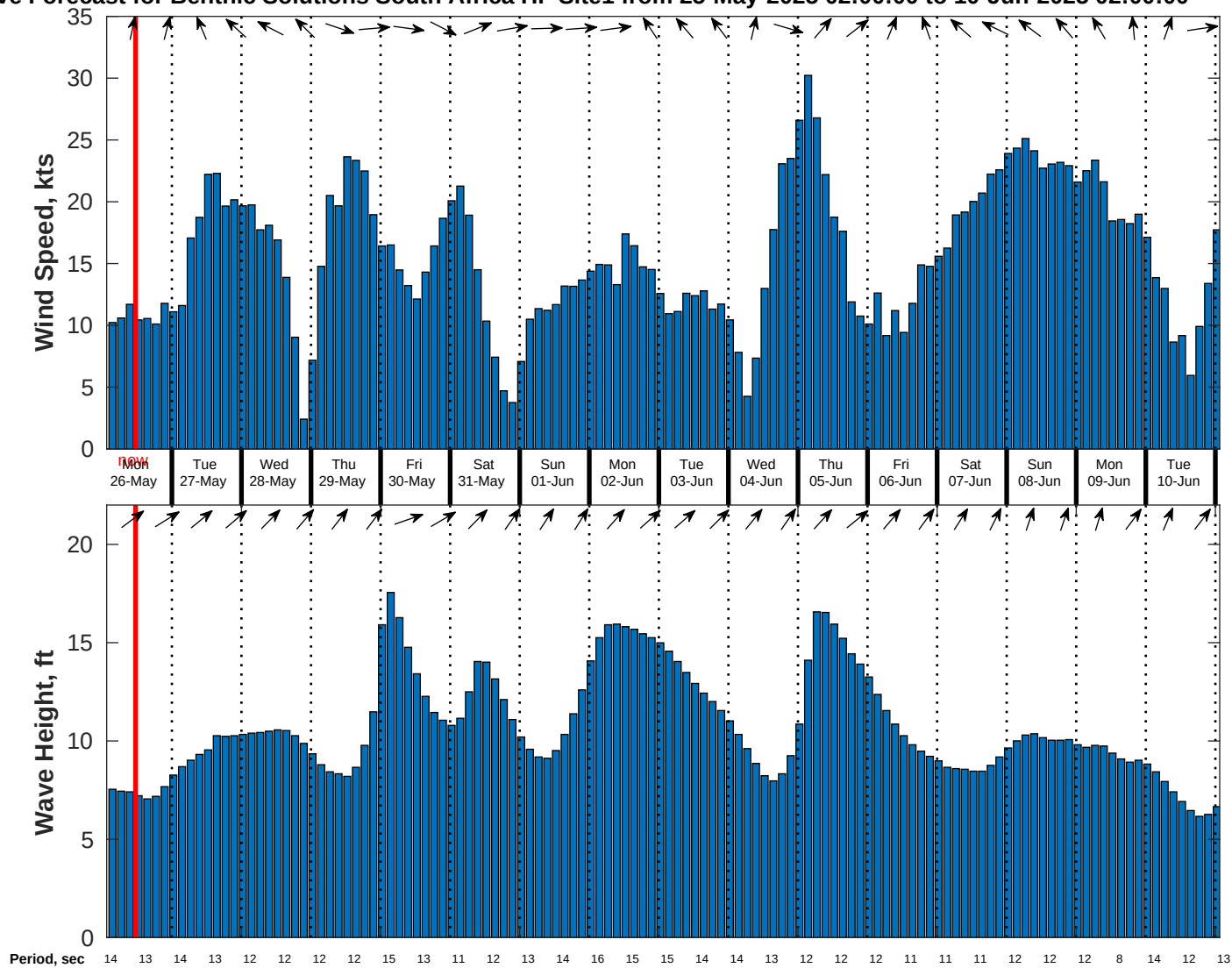
Wind & Wave Forecast for Benthic Solutions South Africa HF Site1 from 25-May-2025 02:00:00 to 10-Jun-2025 02:00:00
