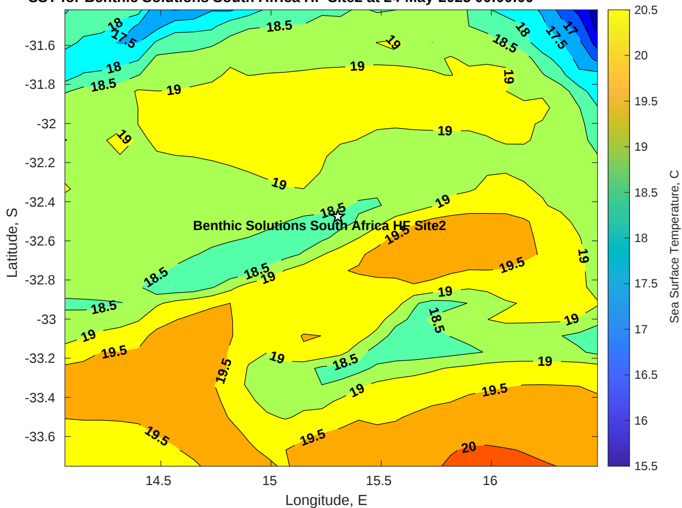
SST for Benthic Solutions South Africa HF Site2 at 24-May-2025 00:00:00
